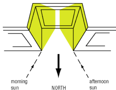
Figure 4.12: Deep north-facing courtyards are overshadowed by the side walls in winter
