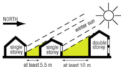
Figure 4.8: Allow adequate distance from obstructions to the north
