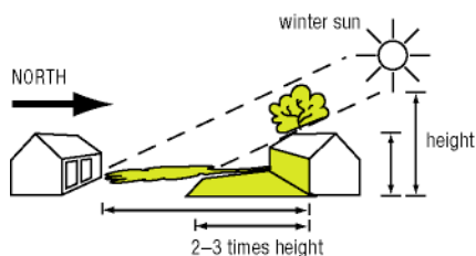
Figure 4.7: Objects cast shadows two to three times their height in winter
