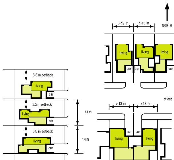
Figure 4.5: Blocks that run north-south and east-west can provide good solar access if minimum boundary widths are provided
