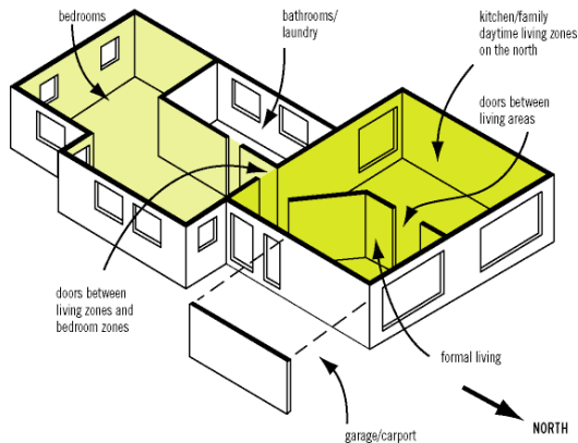
Figure 4.10: Zoning a home for a narrow north-south block
