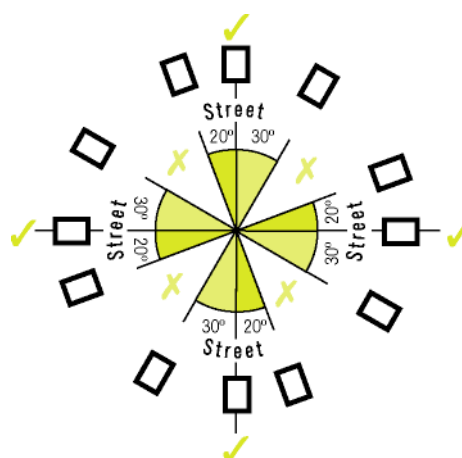
Figure 4.3: Preferred orientation range of lots
