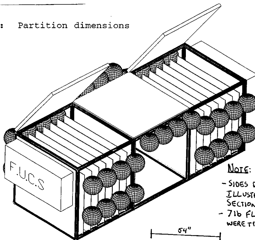
Figure 4b: Mechanical Drawing of the Prototype Cage
