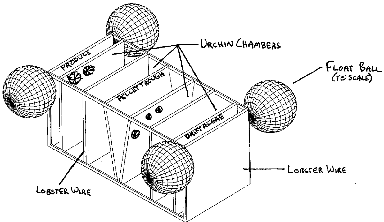
Figure 8: Mechanical Drawing of Modular Slot
