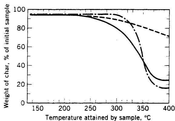
Fig. 12. Portion of dynamic thermogravimetric curves between 130 and 400 °C, with temperature rising 6 °C per minute for wood, lignin, and \alpha -cellulose. — wood, --- lignin, .-.-.- \alpha -cellulose (36).
