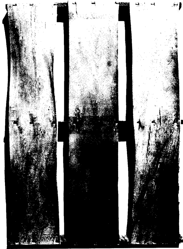
Figure 13.—Top of a berry crate; the two outside pieces contain tension wood but the center does not. Compare the uneven shrinkage and fuzzy appearance of slats with tension wood with the smooth surface of the center slat.
