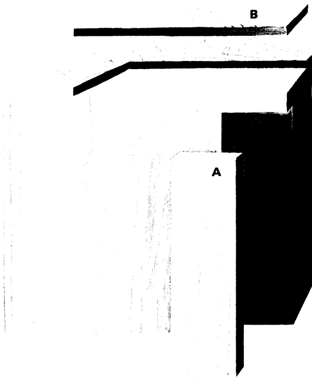
Figure 15.—The slats for the shrinkage test should be cut from a block so that: A, the grain runs parallel to the long dimension, and B, the grain is perpendicular to the long dimension.
