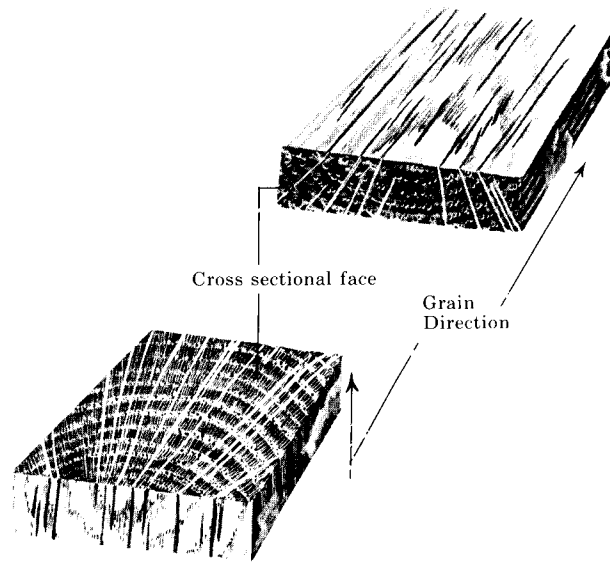
Figure 14.—The two types of blocks required in the liquid penetration test. The upper block has the grain at right angles to the small dimension, while the lower block has the grain parallel to the small dimension.
