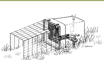
Figure 20b. Bodygrip, cubby set with restricted entry
