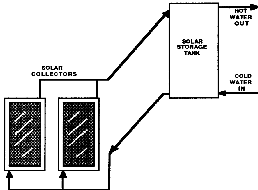
FIGURE 2-14 A Thermosiphon System
