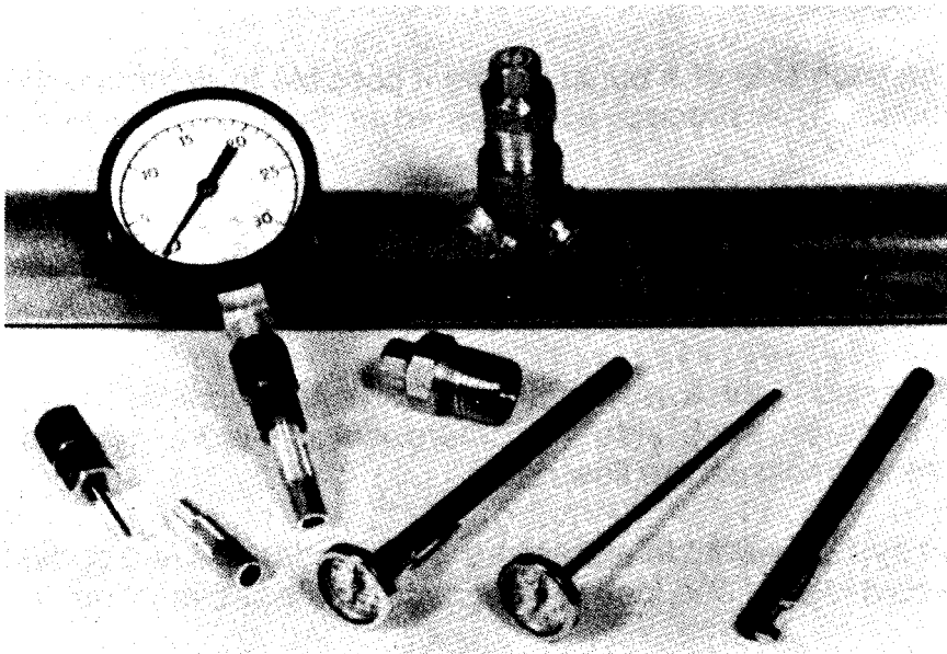
FIGURE 2-51 Insertion Thermometers with PT Plugs
