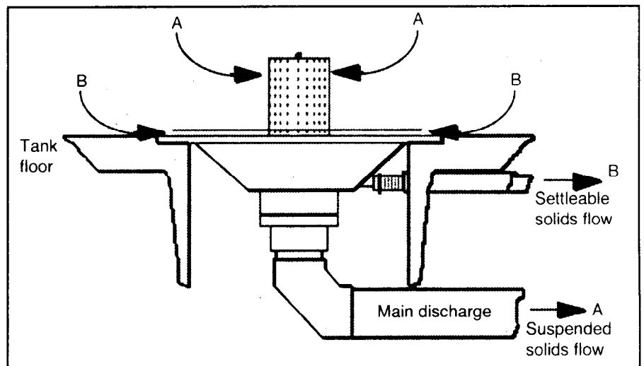
Figure 2. The ECO-TRAP TM particle trap is an advanced double drain design that concentrates much of the settleable solids in only 5 percent of the water flow leaving the fish culture tank (B). (after Hobbs et al., 1997). (ECO-TRAP is a trademark of AquaOptima AS, Pir Senteret, 7005 Trondheim, Norway, U.S. Patent No. 5,636,595.)
