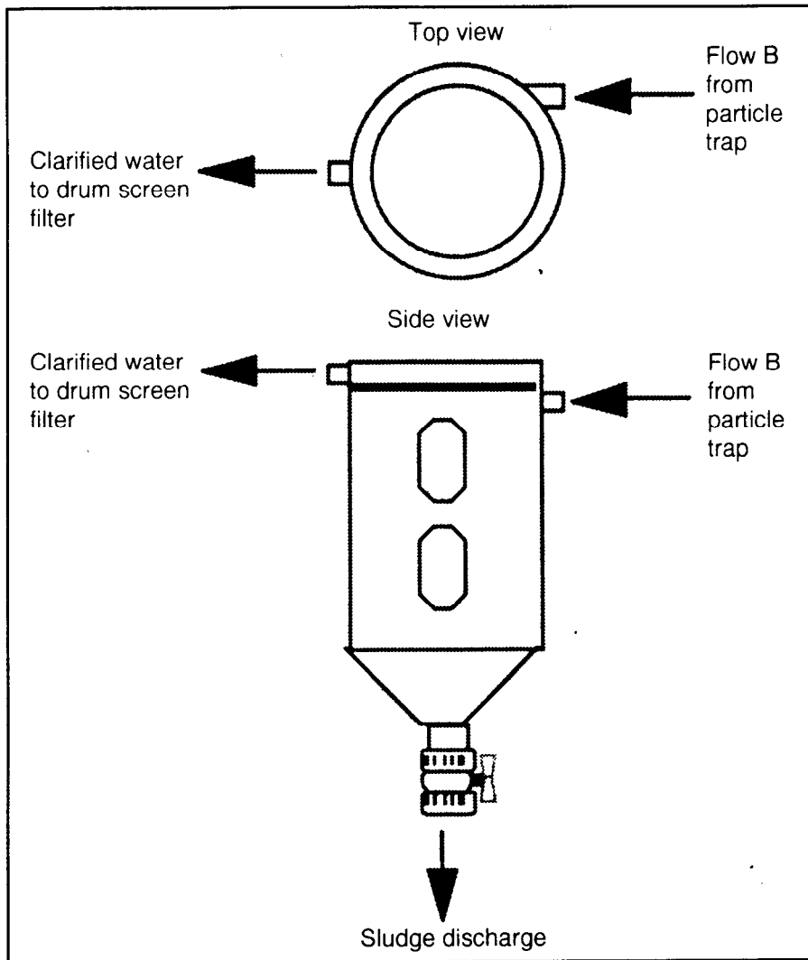
Figure 3. The sludge collector that works in conjunction with the ECO-TRAP™ to remove settled solids from the flow stream B (Fig. 2) (after Hobbs et al., 1997).
