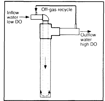
Figure 15. Typical u-tube oxygen diffusion design.
