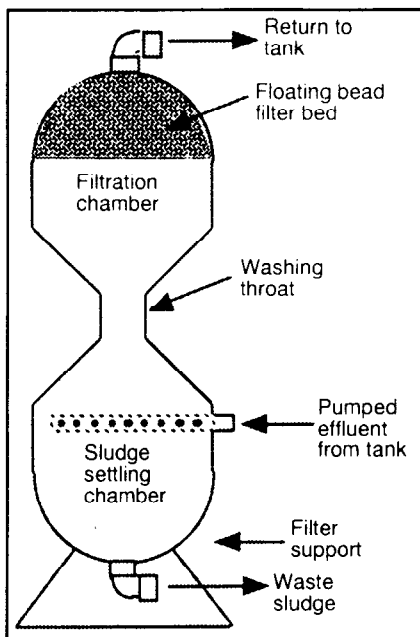
Figure 8. The bubble bead filter operates much like the propeller washed bead filter, except that it backwashes by dropping the filtration medium by gravity through a washing throat. (U.S. Patent No. 5,232,586 by Dr. Ronald Malone, Dept. of Civil Engineering, Louisiana State University)
