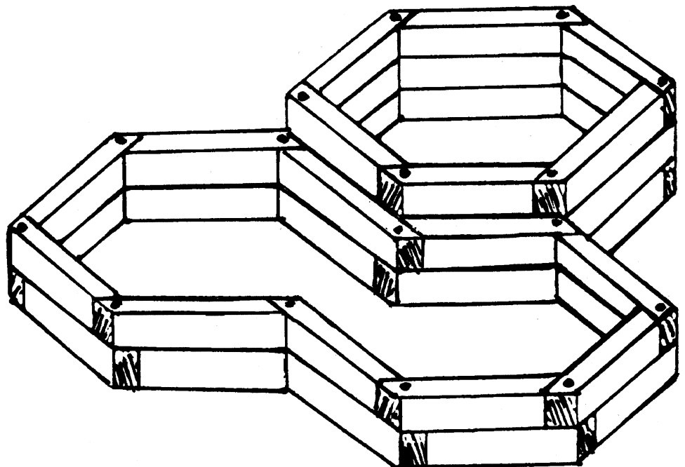
Landscape timbers with liners can be used to construct above ground ponds in any shape.
