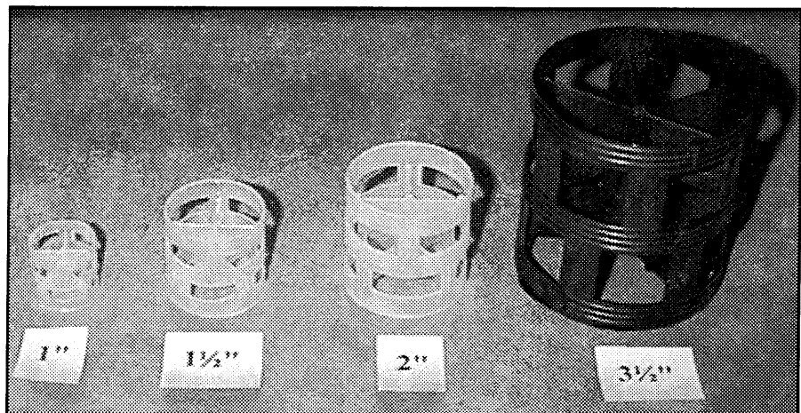
Figure 1. Pall rings of various sizes can be used as media in packed columns.
