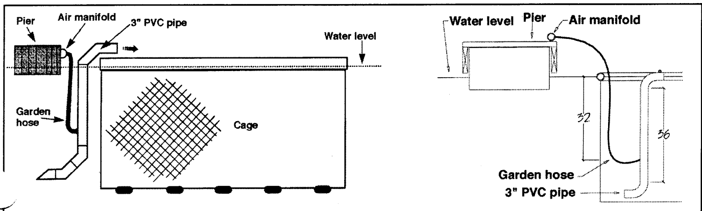
Fig. 5. Cage along a pier with air-lifts mounted over the top of the case (left) and inside the cage (right).
