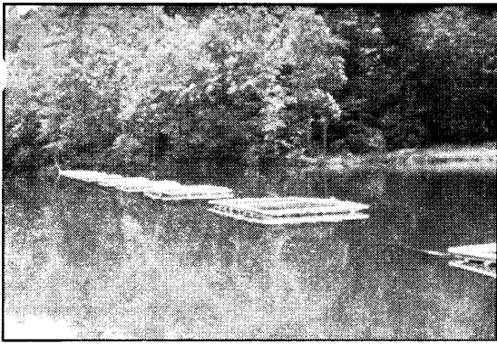
Fig. 4. Cages properly separated across pond with no pier.
