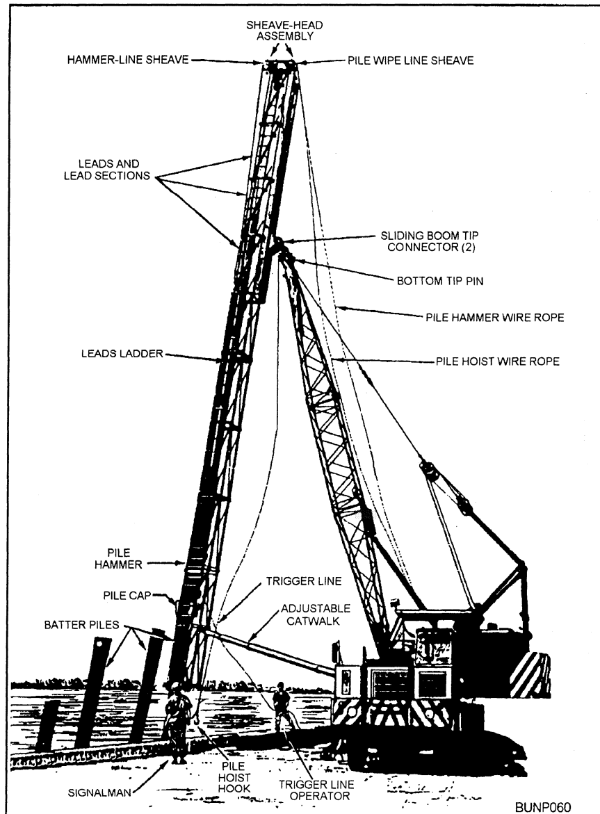
Figure 8-13.—Typical pile-driving operation.
