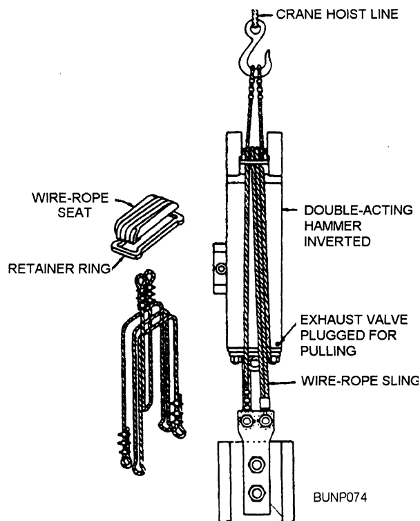
Figure 8-27.—Wire-rope sling used with 5,000-pound airstream hammer to pull piles.
