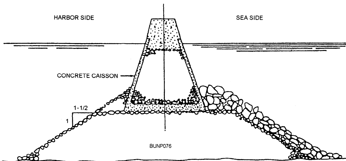
Figure 8-30.—Composite breakwater or jetty.
