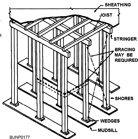
Figure 3-4.—Typical overhead slab form.
