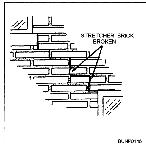
Figure 7-4.—Diagonal movement crack.
