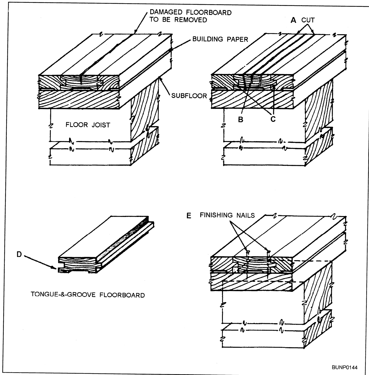
Figure 7-2.—Method of replacing tongue-and-groove flooring.
