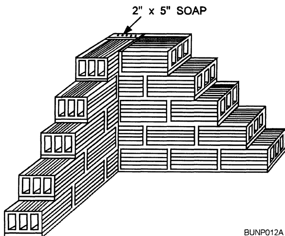
Figure 4-24.—Eight-inch structural clay tile wall.
