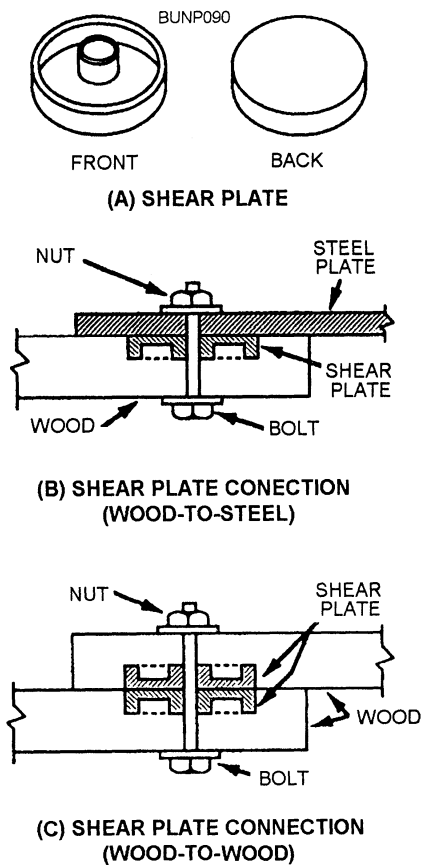
Figure 8-44.—Shear plate and shear-plate joints.
