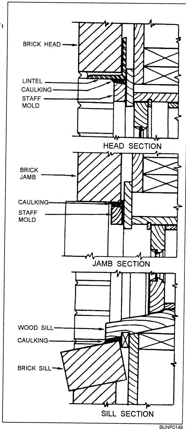
Figure 7-7.—Required caulking around window frames.
