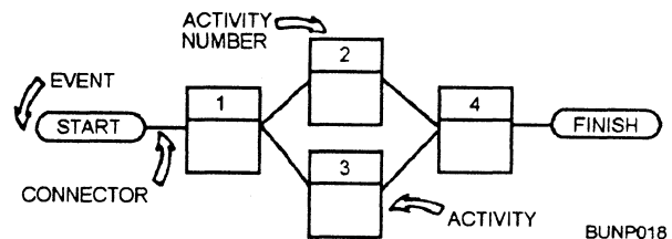
Figure 2-24.—Precedence diagram.
