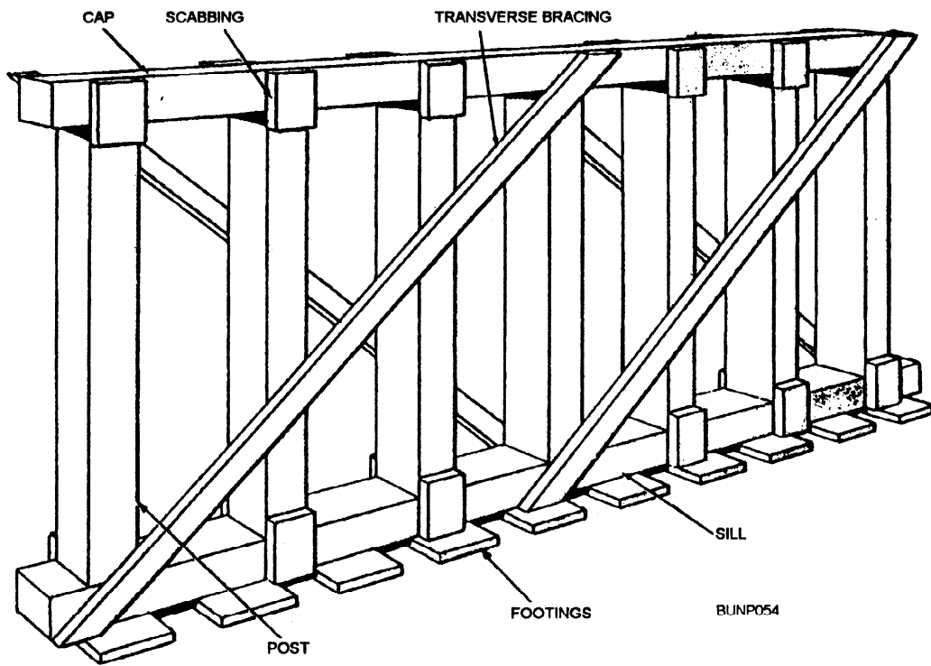
Figure 8-7.—Timber trestle bent.
