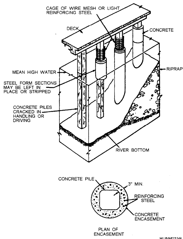
Figure 7-17.—Encasement of damaged piles (metal form).
