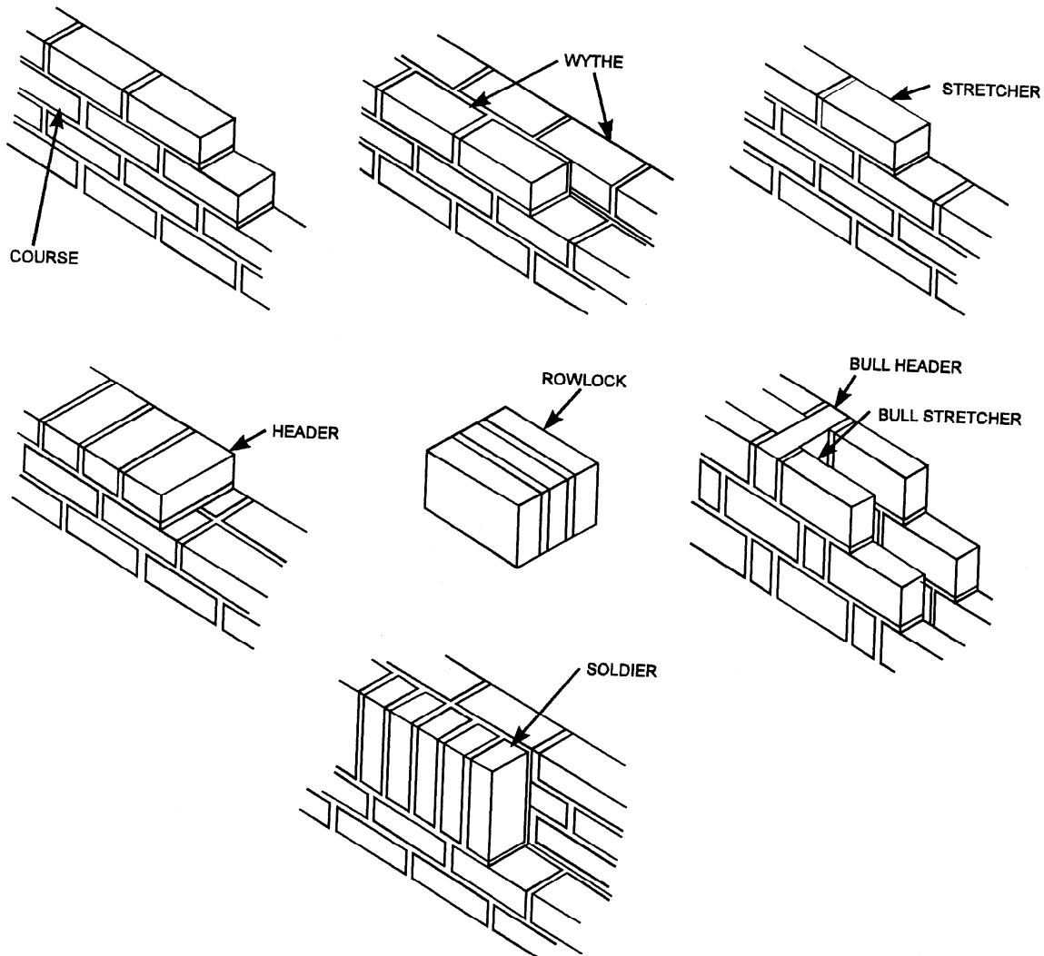
Figure 4-1.—Masonry units.
