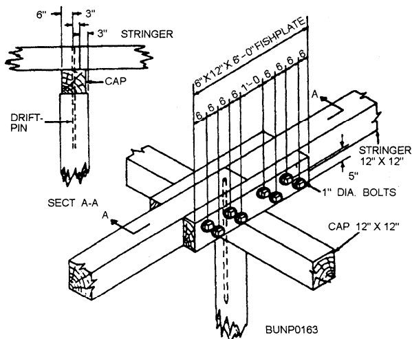
Figure 7-21.—Stringer splice.
