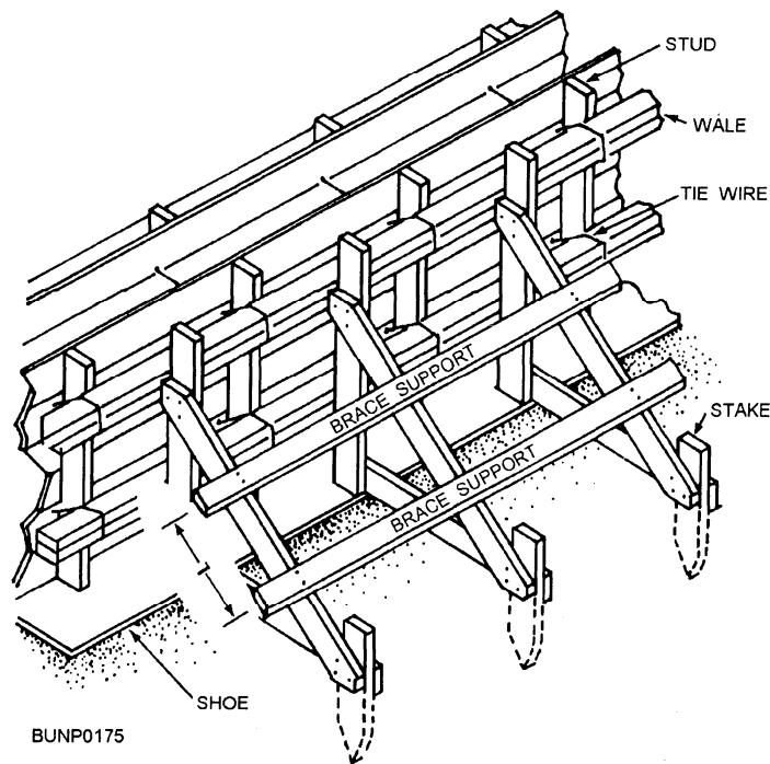
Figure 3-3.—Diagonal bracing supports.
