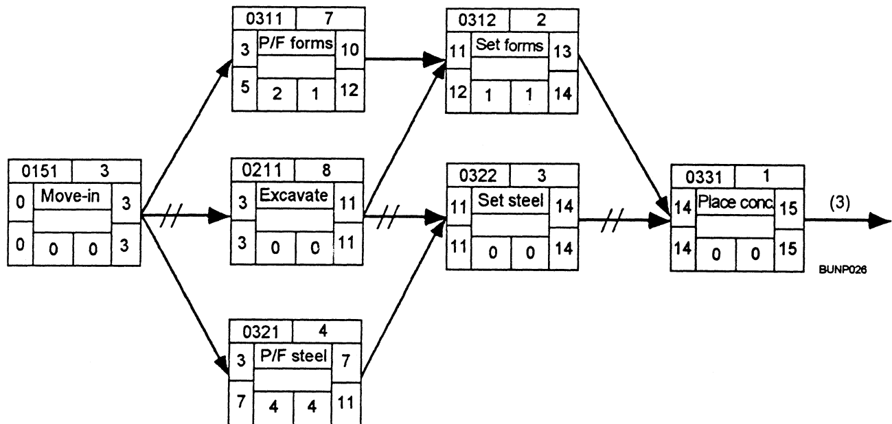
Figure 2-31.—Logic network.
