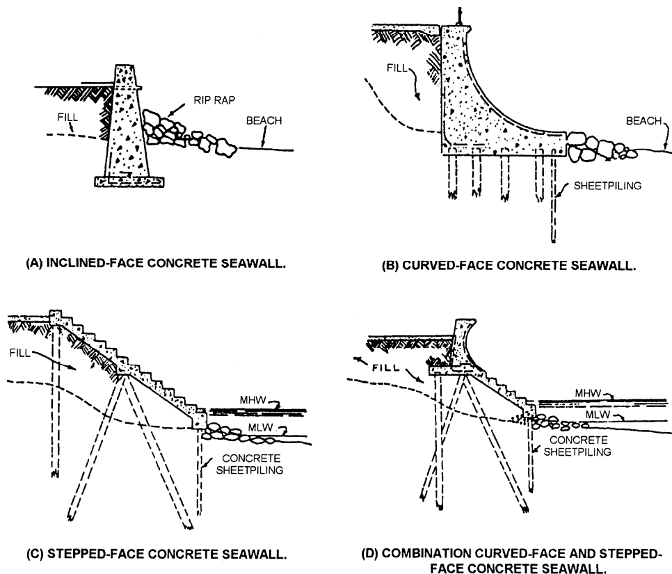
Figure 8-32.—Various types of seawalls.
