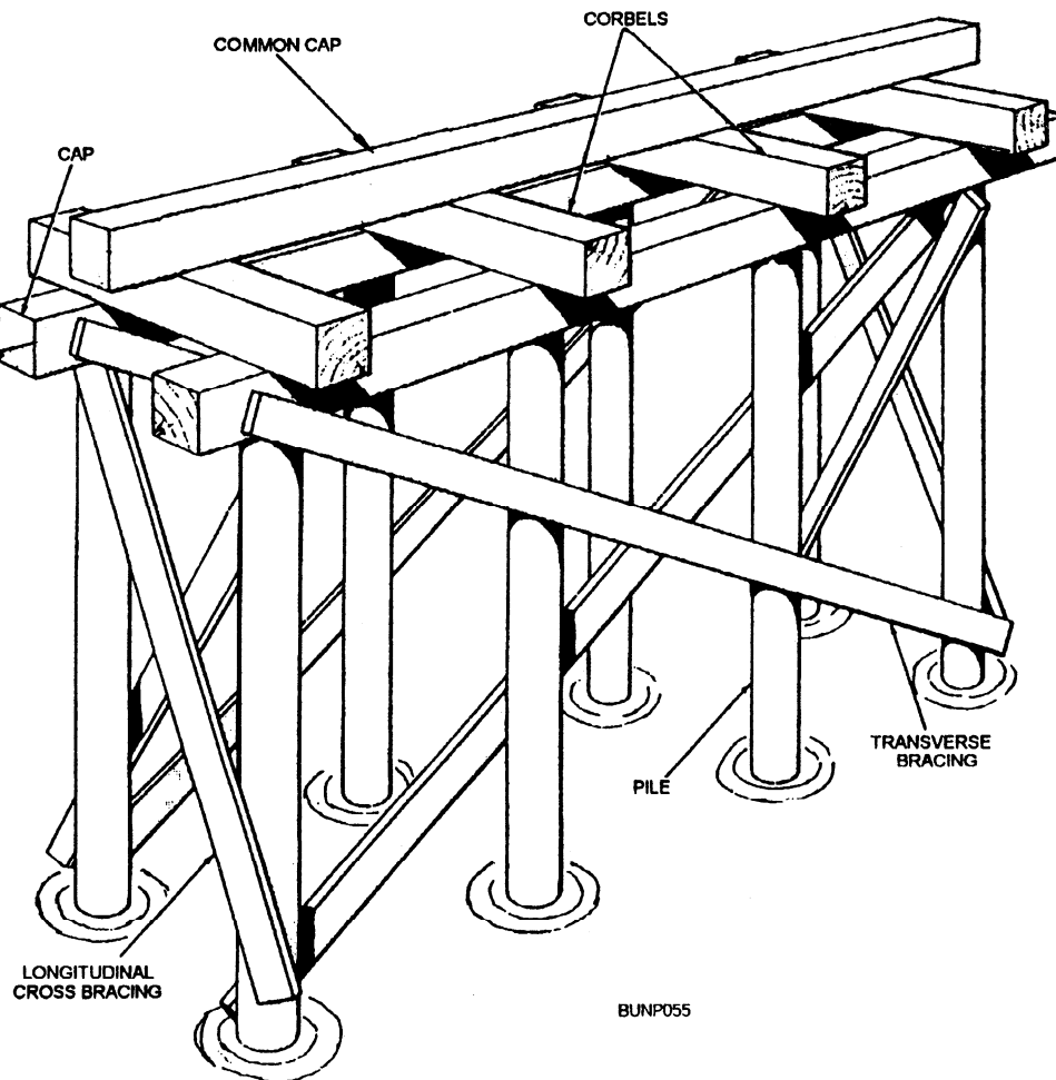
Figure 8-8.—Typical pile pier.
