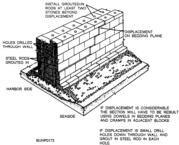
Figure 7-31.—Reinforcing vertical walls.
