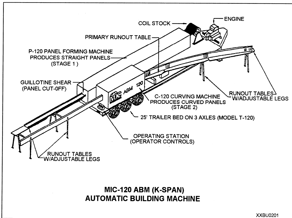
Figure 9-9.—Automatic Building Machine 120.
