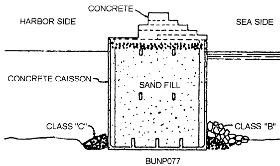
Figure 8-31.—Caisson breakwater or jetty.
