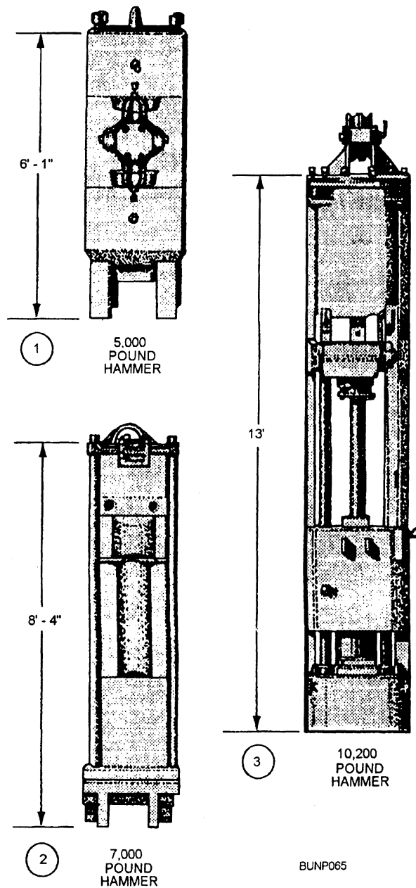
Figure 8-18.—Steam, or pneumatic, pile hammers.
