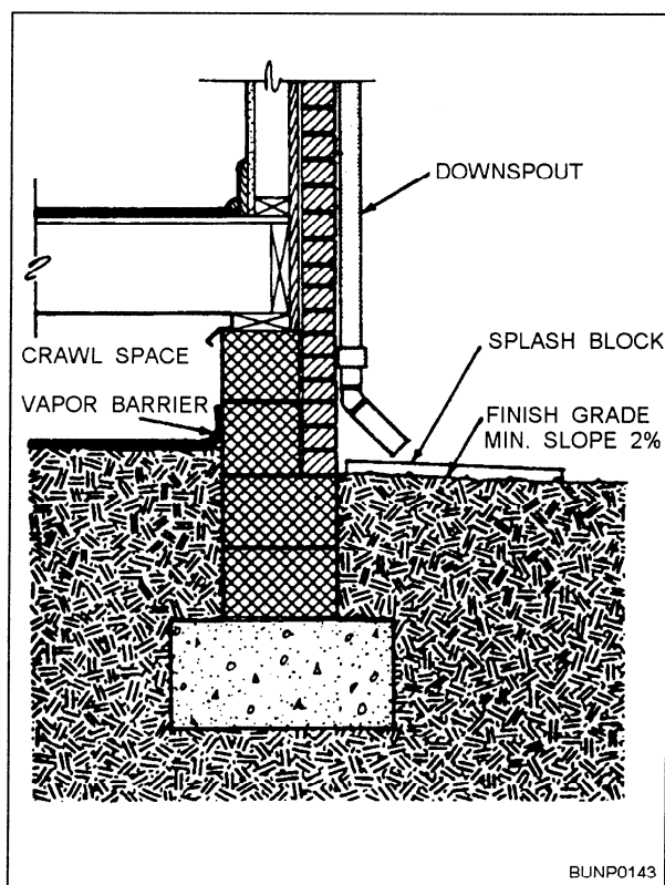
Figure 7-1.—Proper drainage for storm water.
