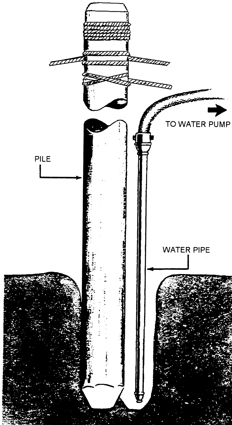
Figure 8-25.—Jetting with a single jet pipe,
