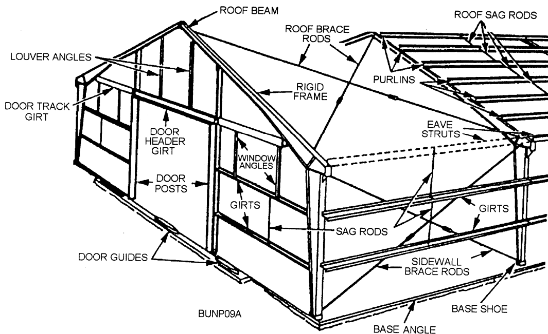
Figure 8-54.—Structural members of a pre-engineered metal building.
