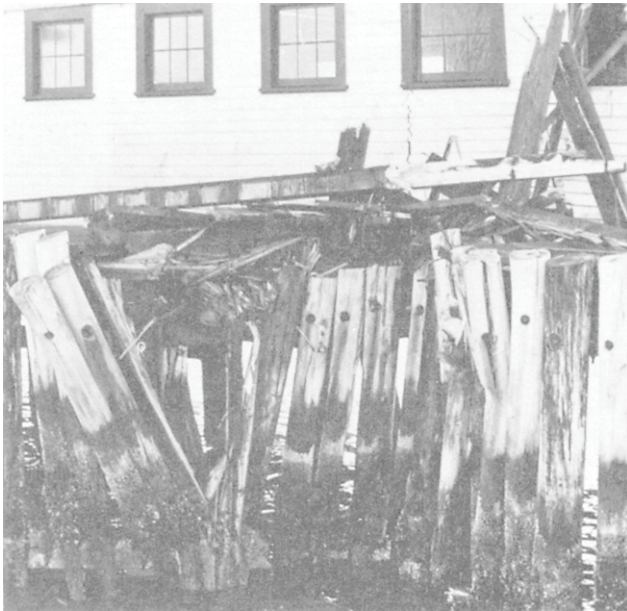
Figure 7-24.—Broken wood piles.
