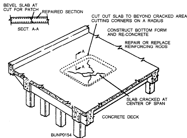
Figure 7-12.—Repair of deck at center of span.
