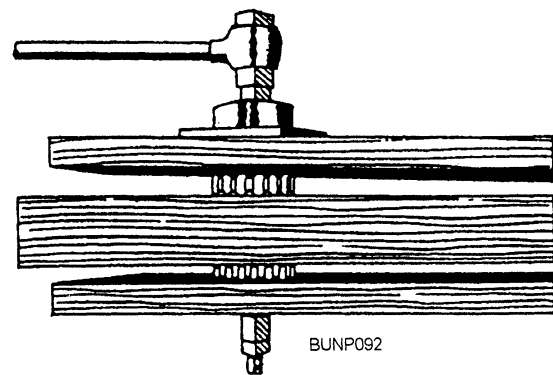
Figure 8-46.—Embedding toothed rings.
