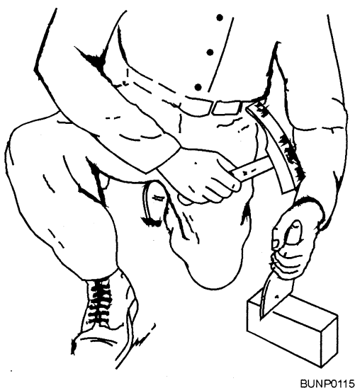
Figure 4-16.—Cutting brick with a chisel.
