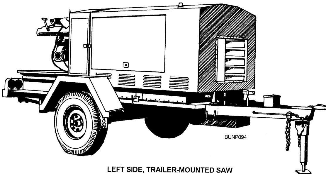
Figure 8-48.—Trailer-mounted radial overarm field saw (front view and side view).
