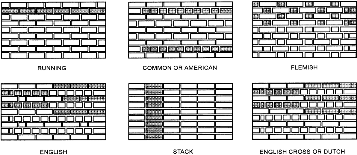
Figure 4-4.—Types of masonry bonds.
