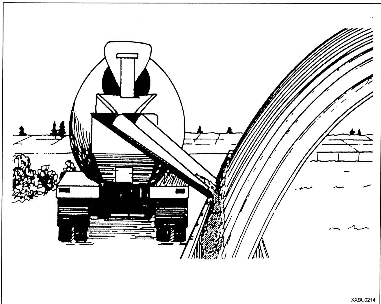
Figure 9-22.—Placement of concrete foundation.
