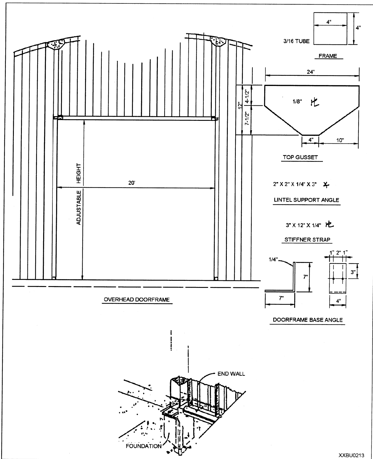
Figure 9-21.—Overhead doorframe.
