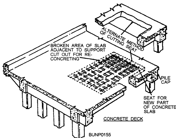
Figure 7-13.—Repair to damaged edge of slab.
