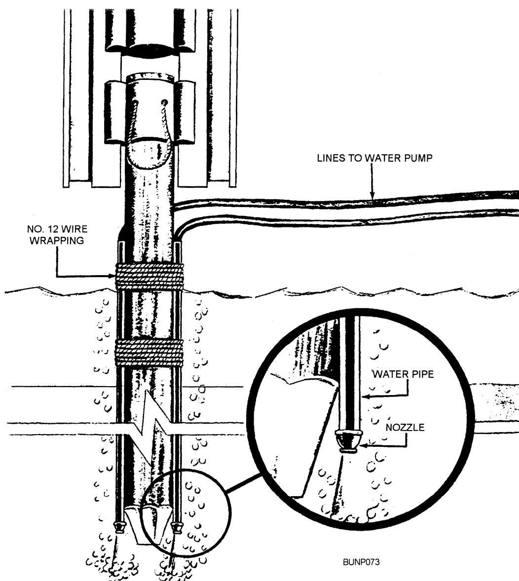
Figure 8-26.—Jetting with two jet pipes.
