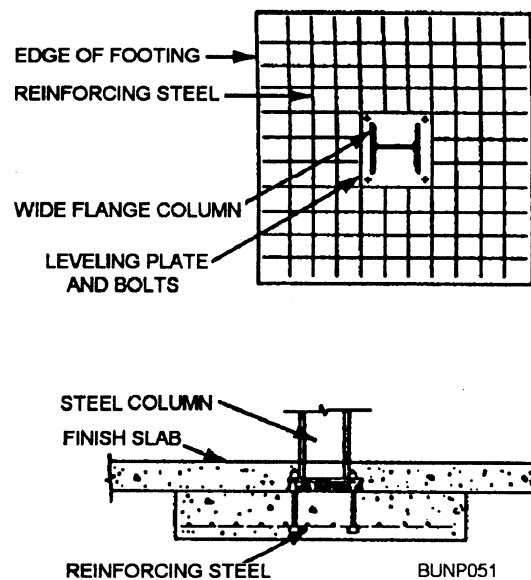
Figure 84.—P1an and section of a typical spread footing.
