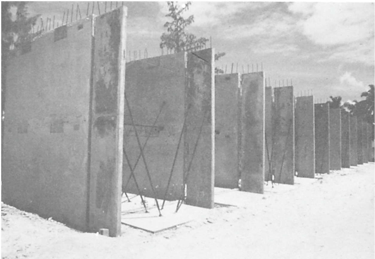
Figure 3-19.—Precast panels in positions.
