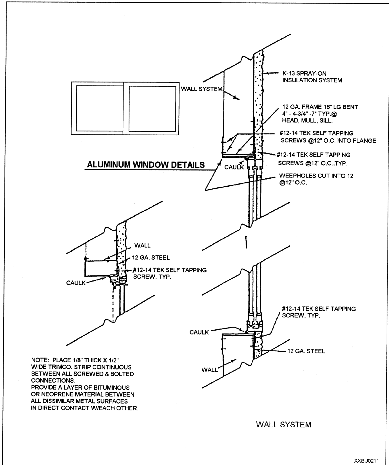
Figure 9-19.—Aluminum window installation.
