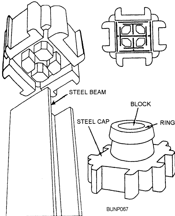
Figure 8-20.—H-beam pile-driving cap.
