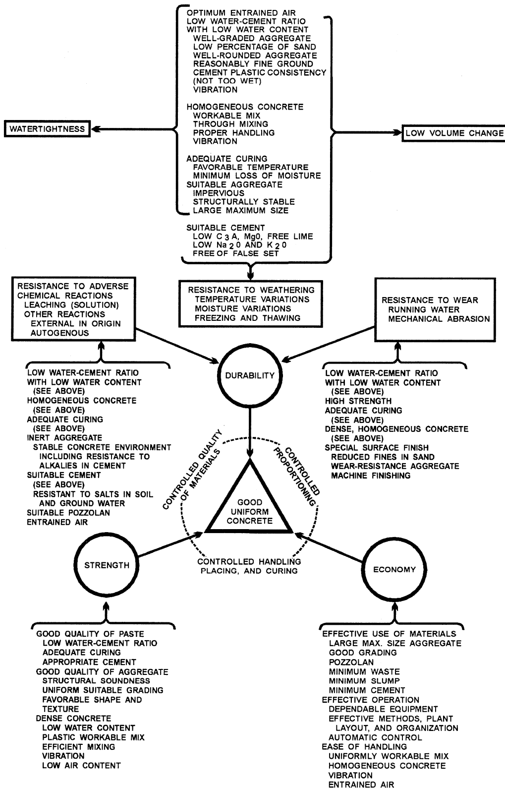
Figure 3-13.—Concrete properties.
