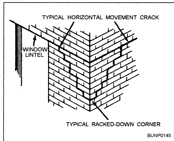
Figure 7-3.—Typical horizontal movement and racked-down corner cracks.
