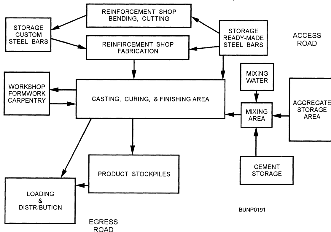
Figure 3-21.—Layout of prefab yard.
