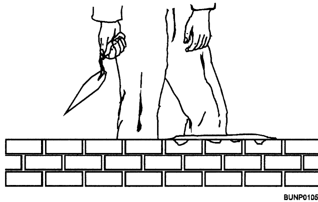
Figure 4-6.—Correct way to hold a trowel.
