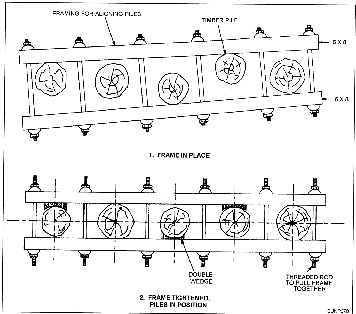
Figure 8-23.—Straightening frame.
