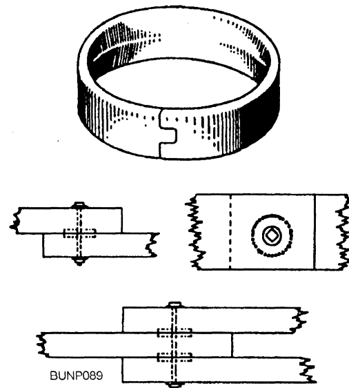
Figure 8-43.—Split ring and split-ring joints.
