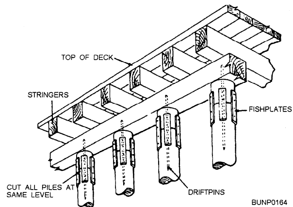
Figure 7-22.—Replacing top of piles.
