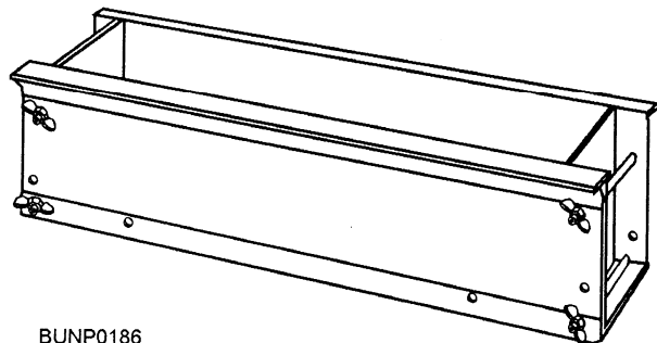
Figure 3-14.—Test beam mold.
