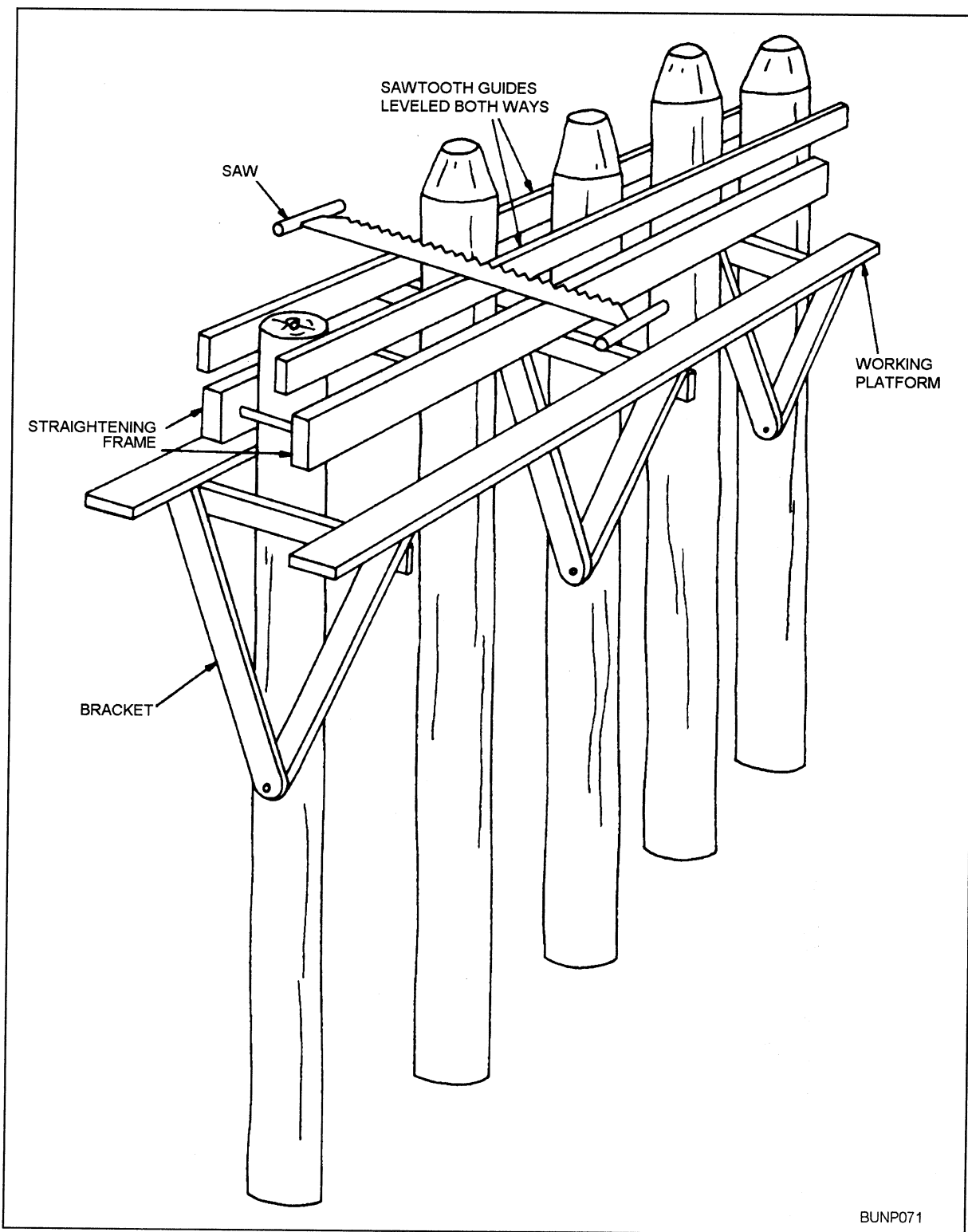
Figure 8-24.—Cutting timber pile bent to final height.
