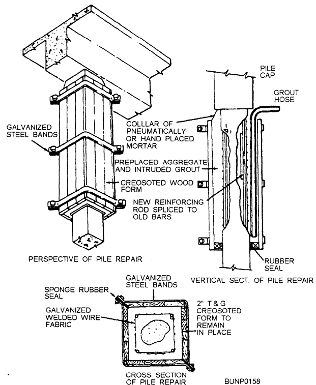
Figure 7-16.—Encasement of damaged piles (wood form).
