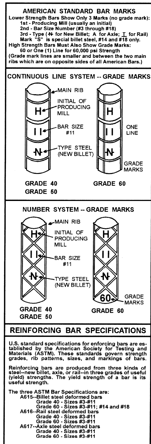
Figure 3-8.—American standard reinforcing steel bar marks.
