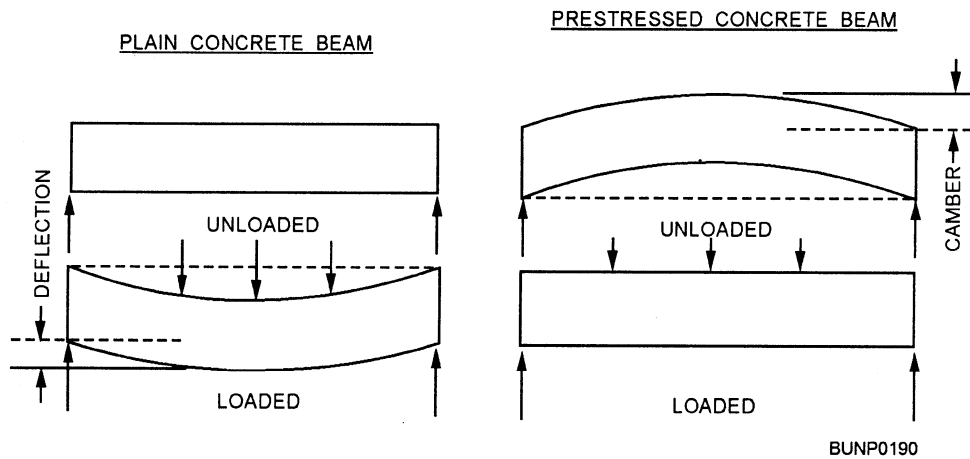
Figure 3-20.—Comparison of plain and prestressed concrete beams.
