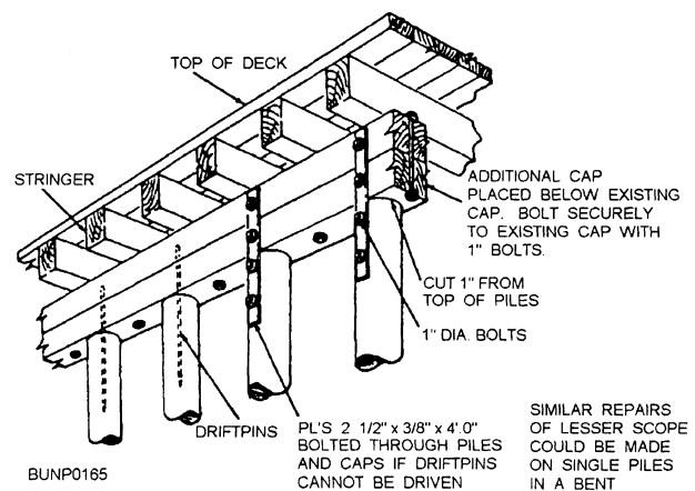
Figure 7-23.—Repair of top of piles.
