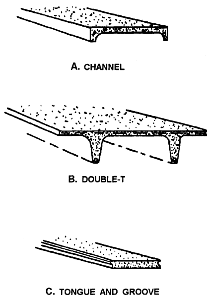
Figure 3-17.—Typical precast panels.
