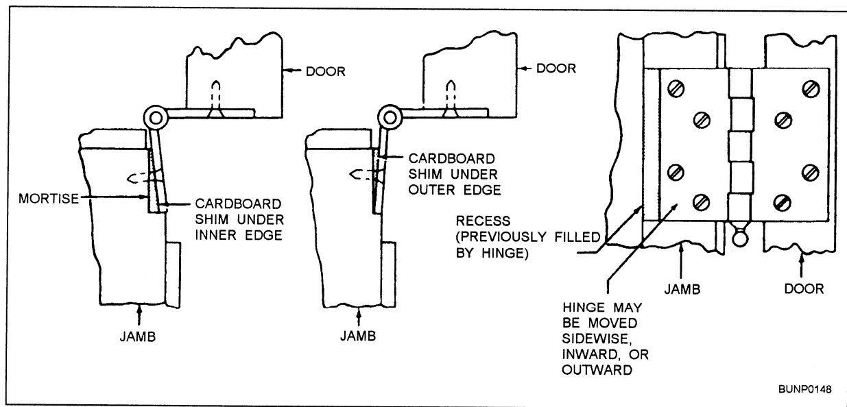
Figure 7-6.—Hinge adjustment for binding or sticking doors.
