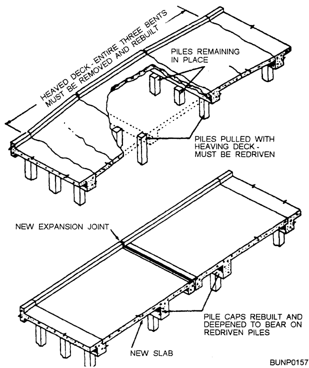
Figure 7-15.—Piles pulled by heaving deck.
