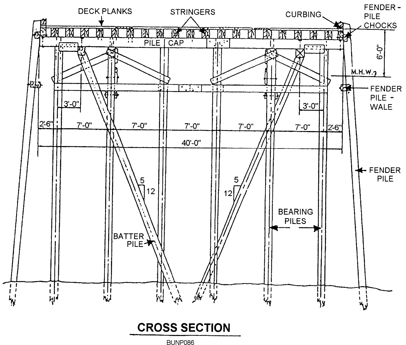
Figure 8-40.—Cross section of an advanced-base timber pier.
