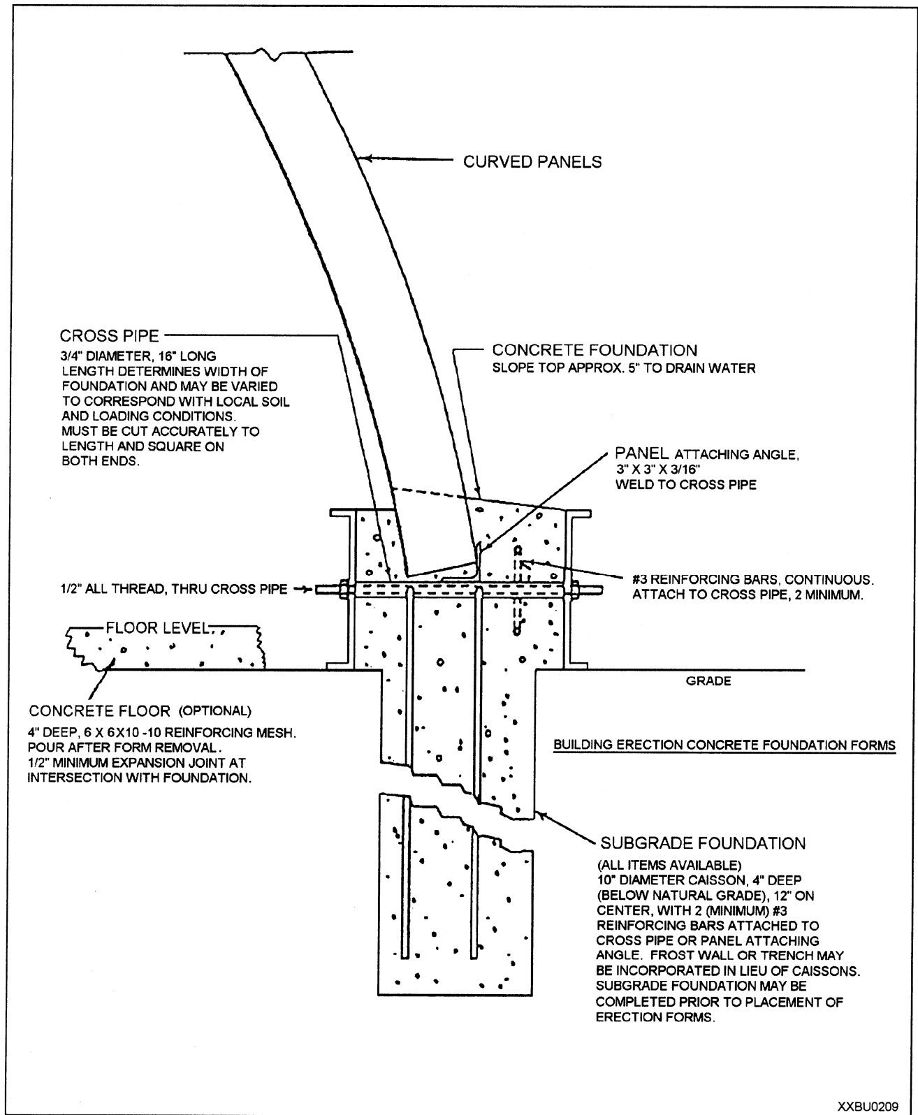
Figure 9-17.—Concrete foundation.
