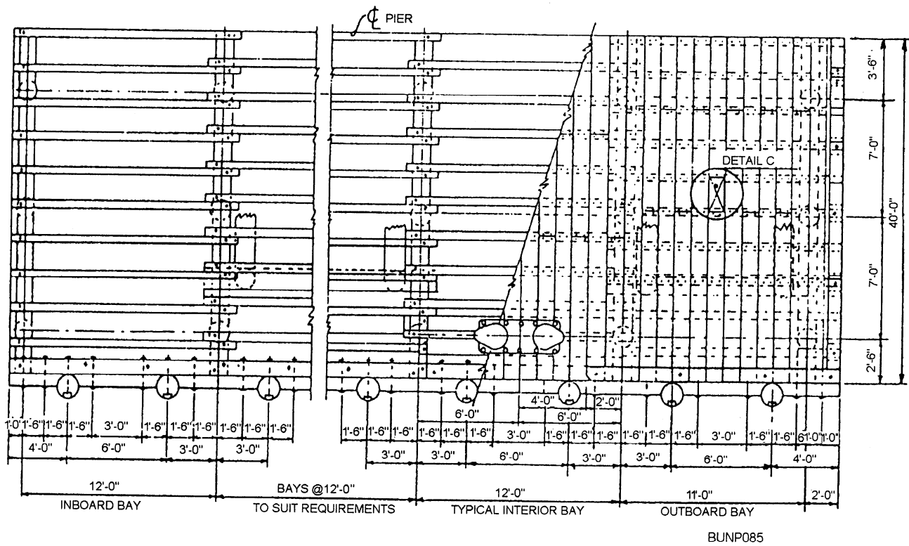
Figure 8-39.—Part plan of an advanced-base timber pier.
