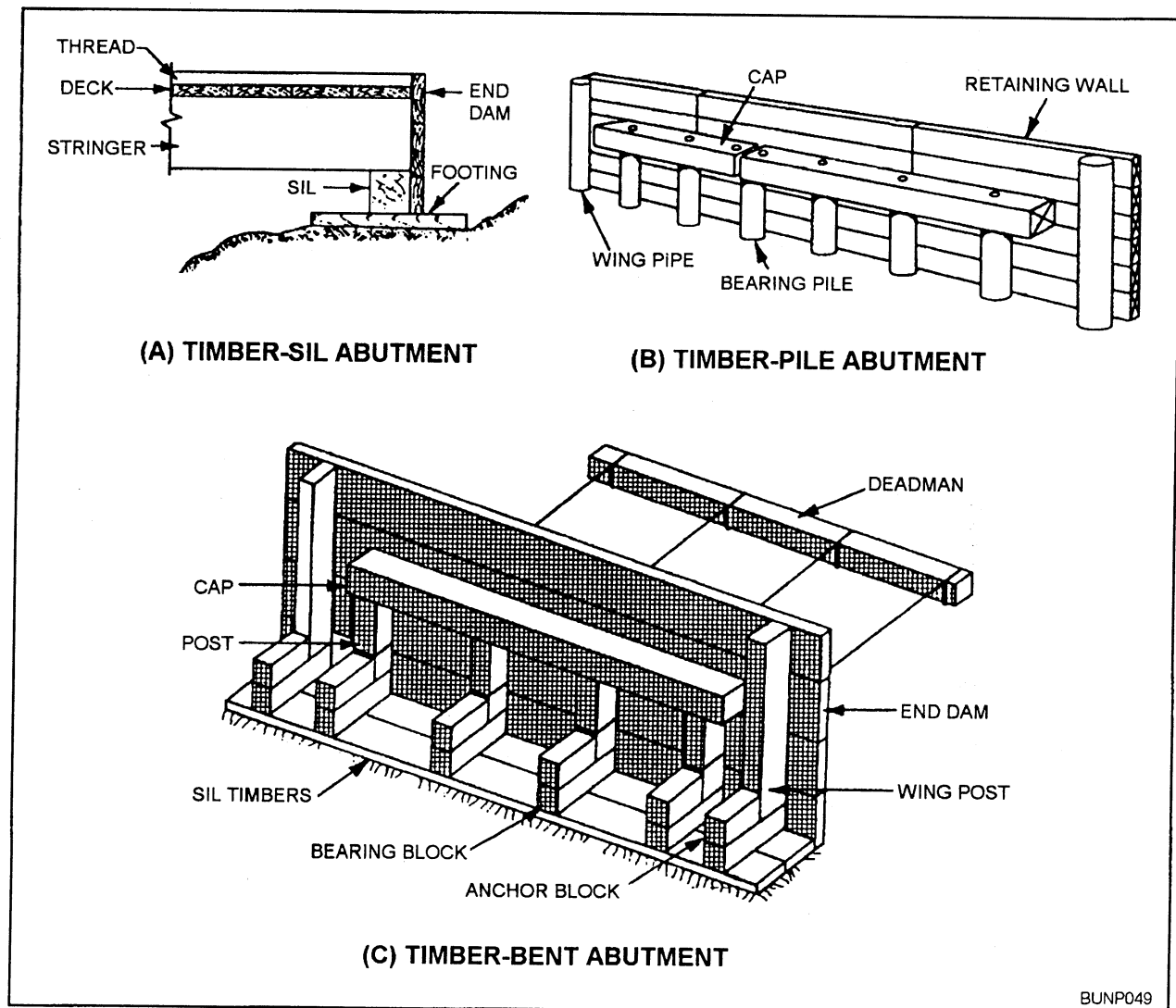
Figure 8-2.—Types of fixed-bridge abutments.
