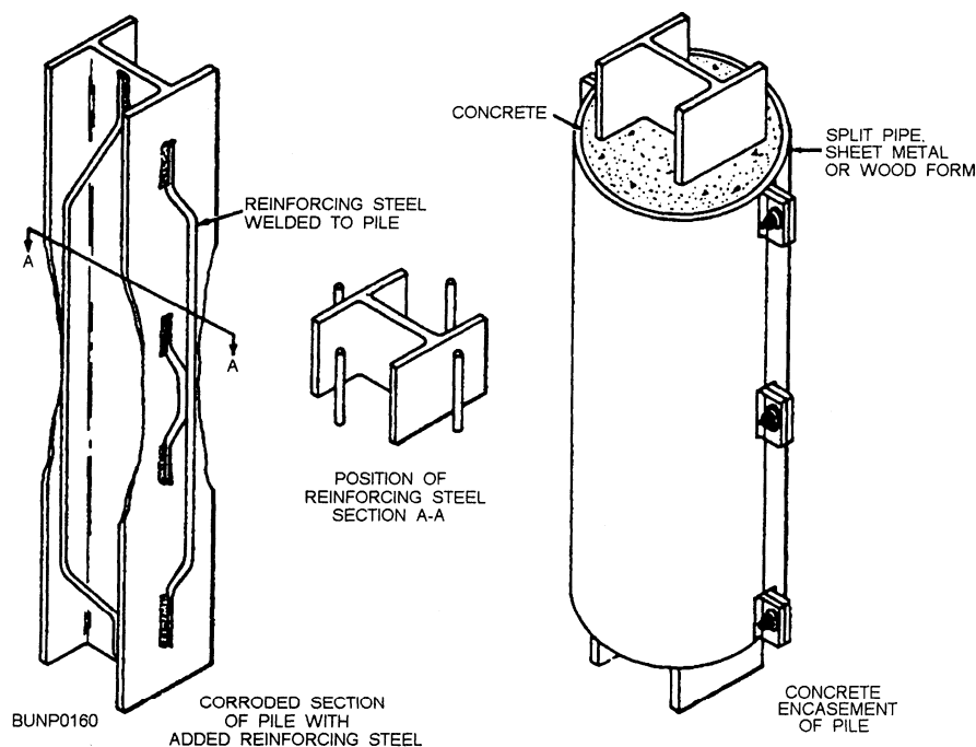
Figure 7-18.—Concrete encasement of steel pile.
