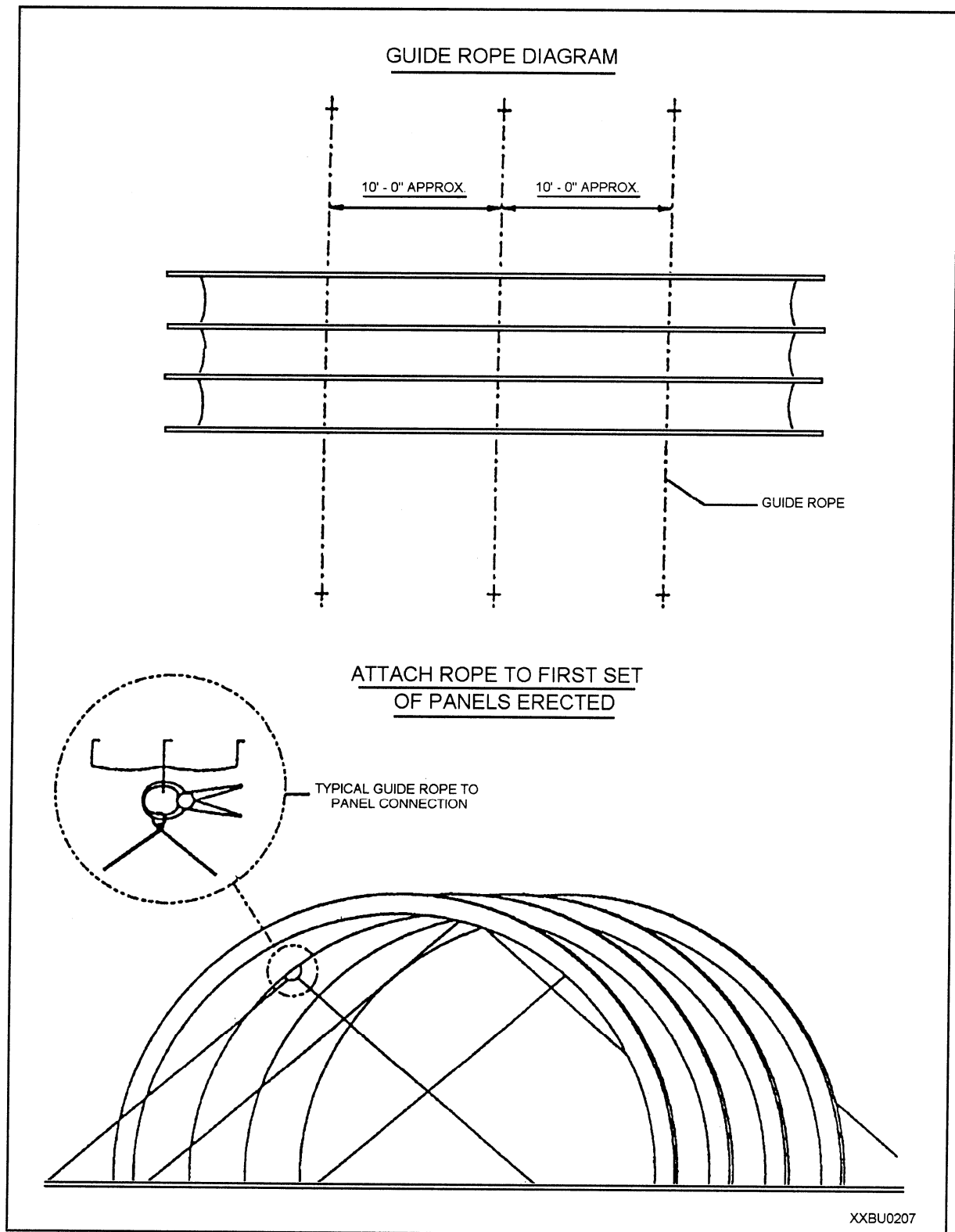
Figure 9-15.—Guide rope diagram.
