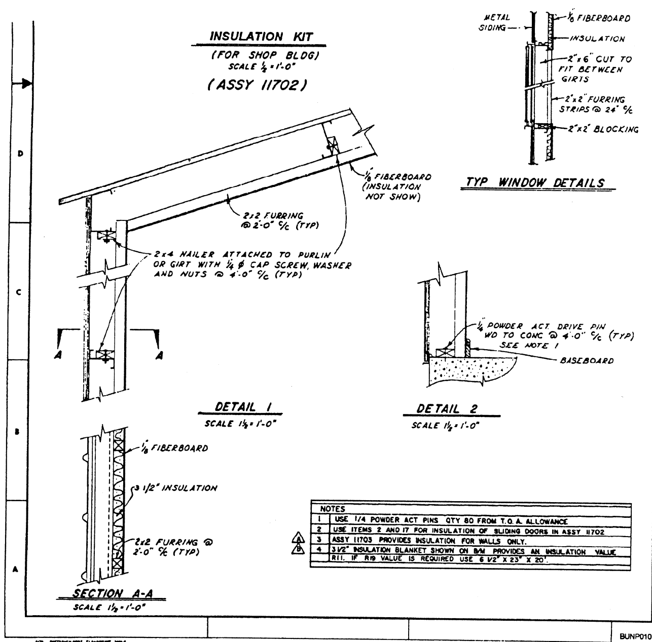
Figure 2-10.—Sectional view.
