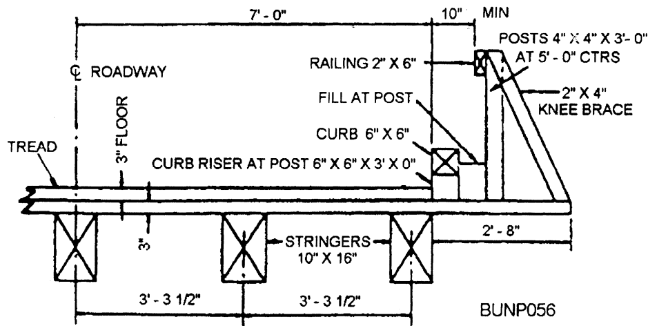
Figure 8-9.—Details of a superstructure of a timber trestle.
