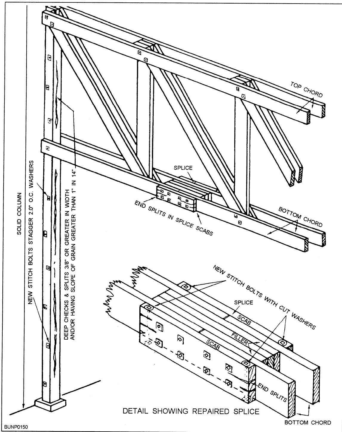
Figure 7-8.—Repair of minor splits using stitch bolts.
