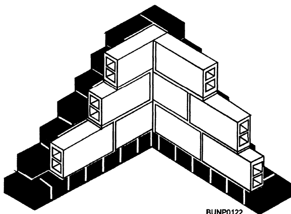
Figure 4-23.—Structural tile used as a backing for bricks.
