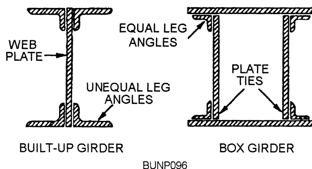
Figure 8-50.—Typical built-up girders.
