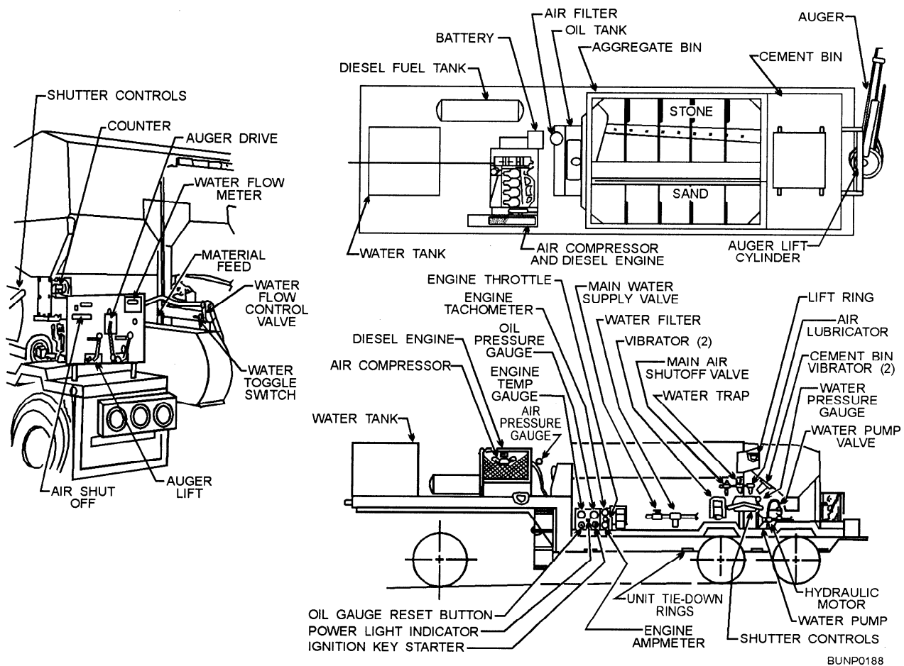
Figure 3-16.—Mobile concrete mixer plant.
