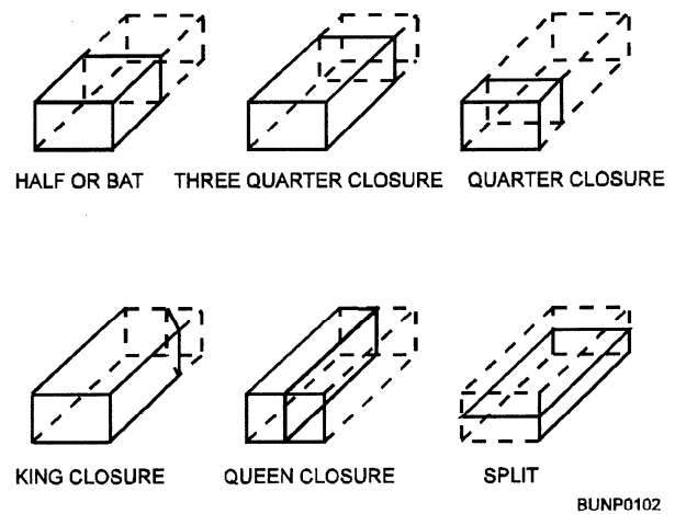
Figure 4-3.—Common cut brick shapes.
