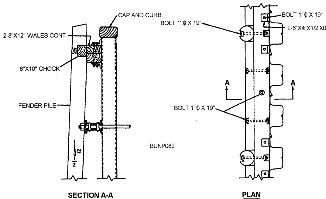
Figure 8-36.—Cap and fender pile for bulkhead.
