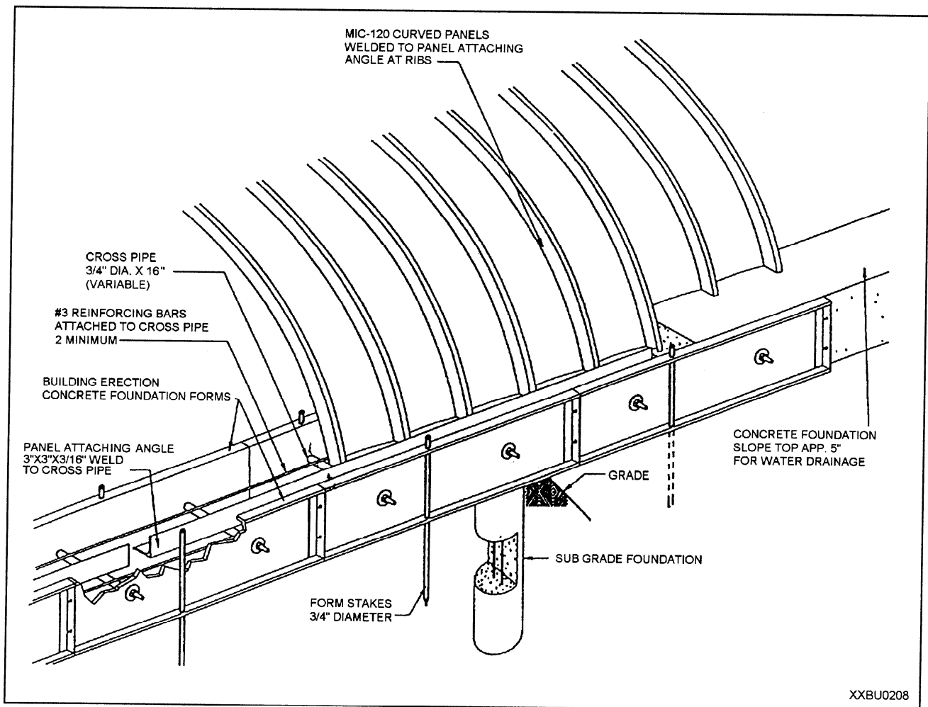
Figure 9-16.—Building foundation concept.
