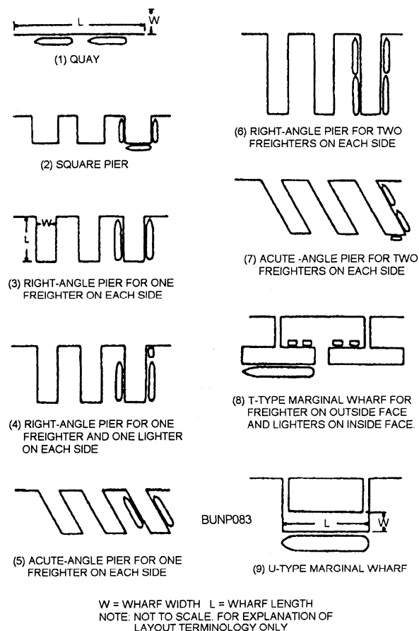
Figure 8-37.—Types of wharfage structures.
