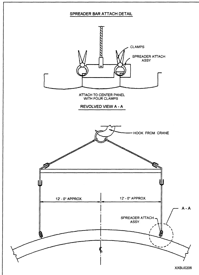
Figure 9-14.—Spreader bar attachment.
