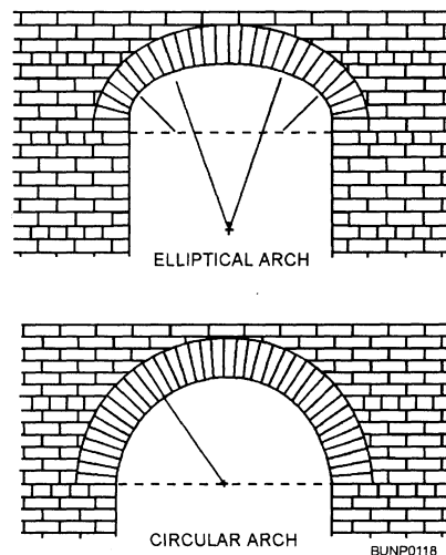
Figure 4-19.—Common arch shapes.
