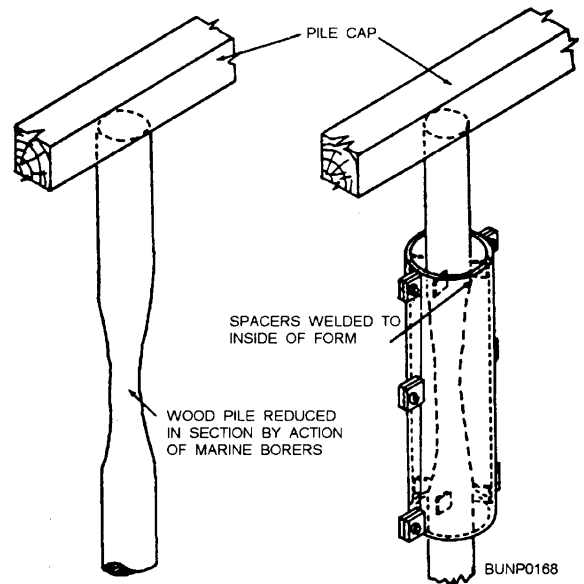
Figure 7-26.—Concrete encasement of short section of wood pile.
