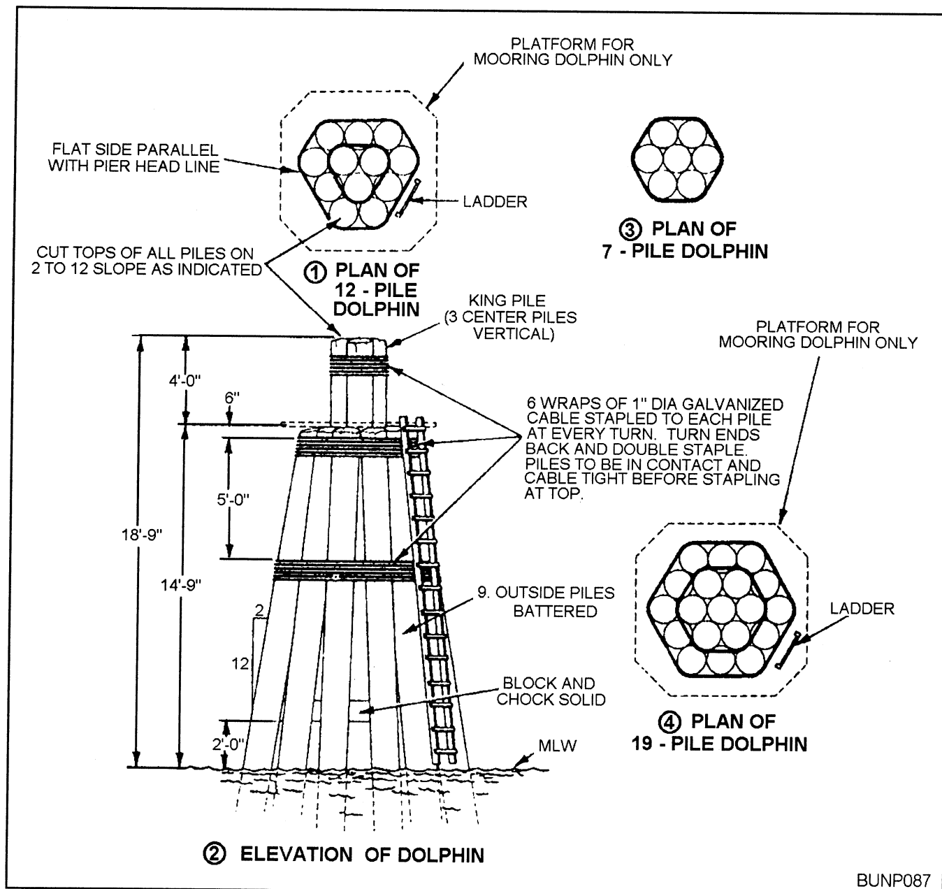
Figure 8-41.—Typical Dolphin Plan.
