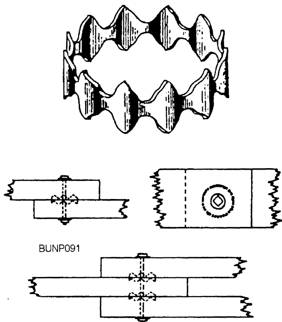
Figure 8-45.—Toothed ring and toothed-ring joints.
