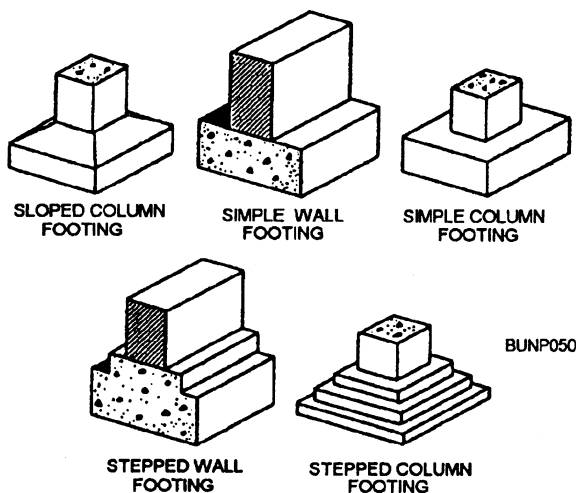
Figure 8-3.—Common wall and column foundations.
