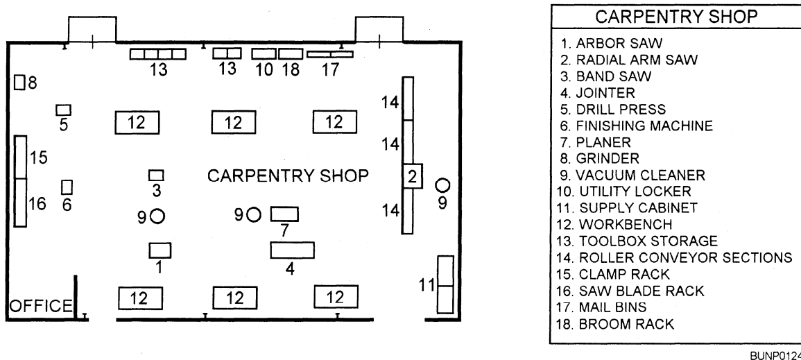
Figure 5-1.—Typical layout of a carpentry shop.
