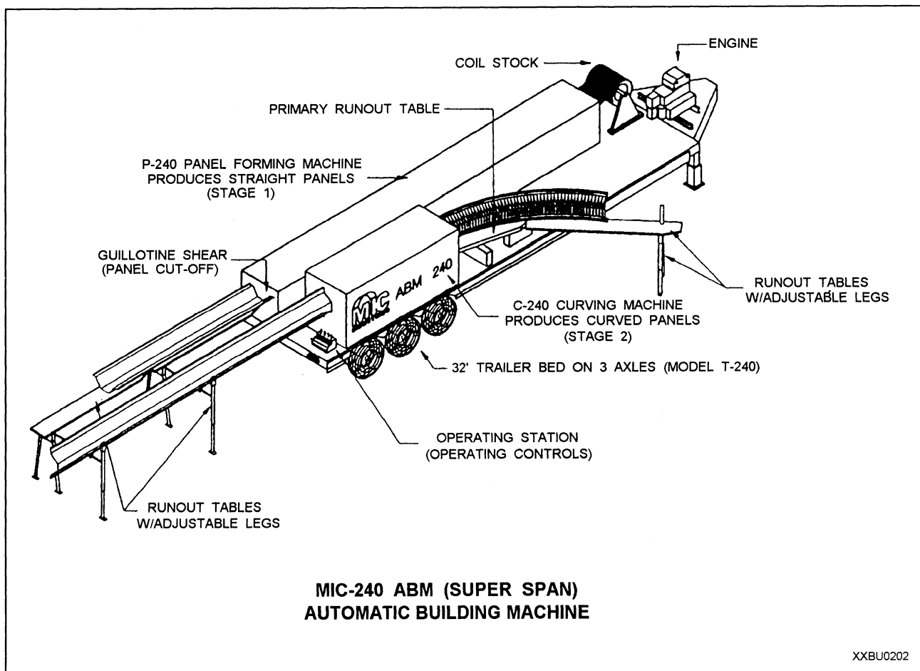
Figure 9-10.—Automatic Building Machine 240.
