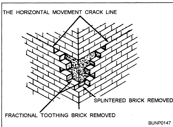
Figure 7-5.—Damaged brick removal.
