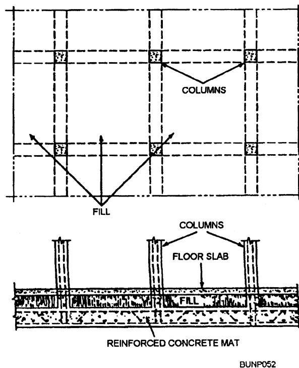
Figure 8-5.—Plan and section of a mat foundation.
