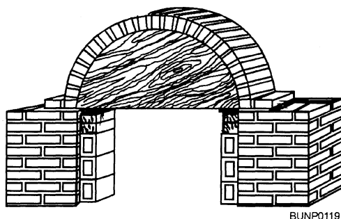
Figure 4-20.—Using a template to construct an arch.
