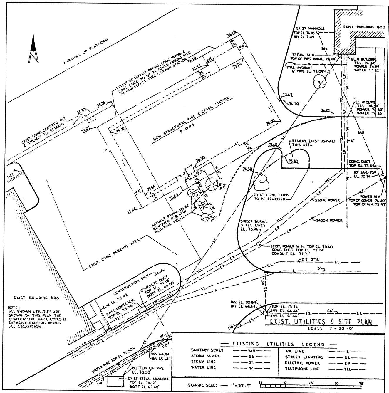
Figure 2-5.—Site plan.
