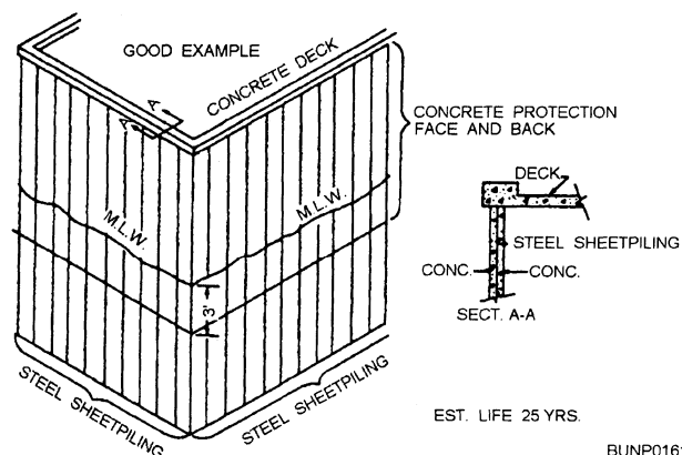
Figure 7-19.—Concrete encasement of steel sheet pile.
