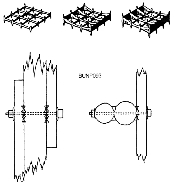
Figure 8-47.—Spike grids and spike-grid joints.
