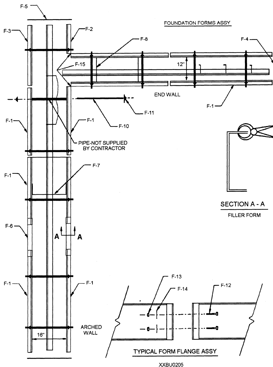
Figure 9-13.—Simple form assembly.
