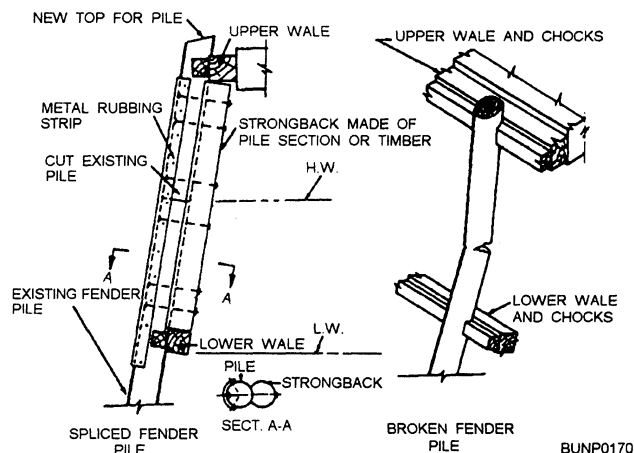
Figure 2-28.—Fender pile repair.
