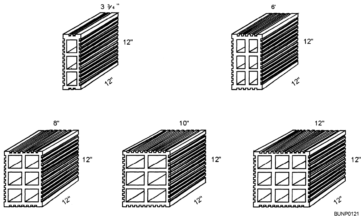
Figure 4-22.—Standard shapes of end-construction building tiles.
