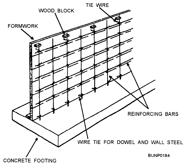
Figure 3-12.—Steel in place in a wall.
