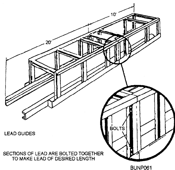
Figure 8-14.—Assembly of 10- and 20-foot sections.
