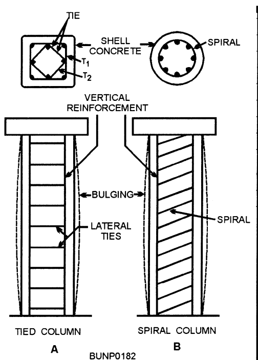
Figure 3-10.—Reinforced concrete columns.
