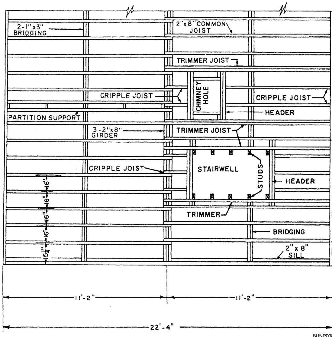
Figure 2-8.—Floor framing plan.
