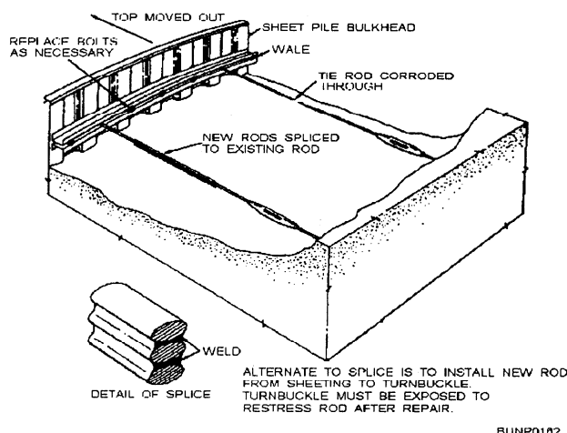
Figure 7-20.—Repair of tie rods.
