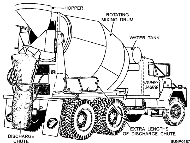
Figure 3-15.—Transit mixer.
