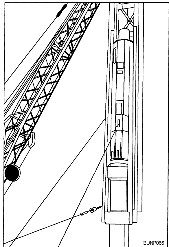
Figure 8-19.—Diesel pile hammer.
