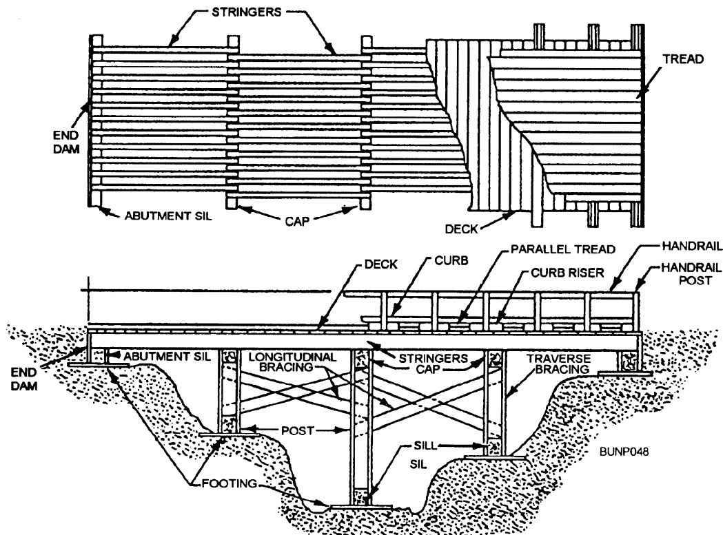
Figure 8-1.—A multispan (trestle-bent) bridge.
