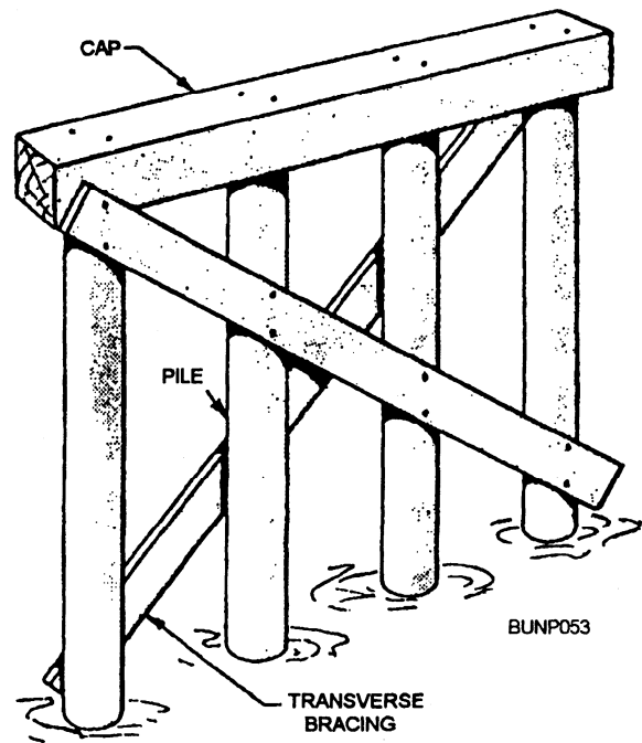
Figure 8-6.—Typical pile bent.
