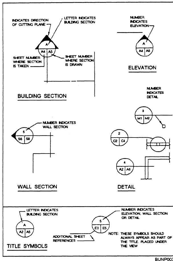
Figure 2-3.—Symbols used to identify sections, elevations, and details.
