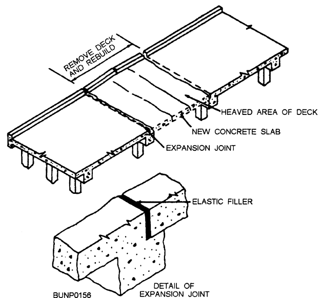
Figure 7-14.—Heaving of concrete deck.
