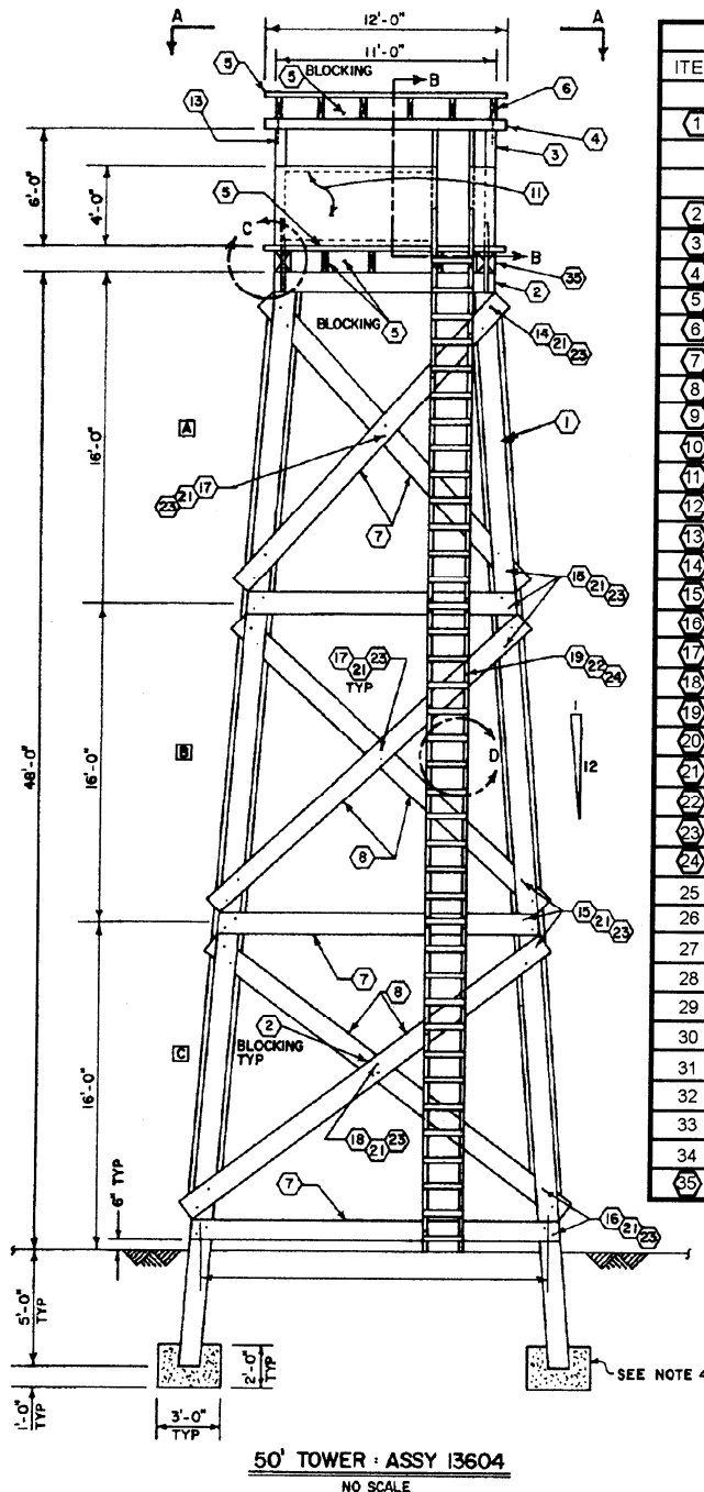
Figure 9-26.—Tower.
