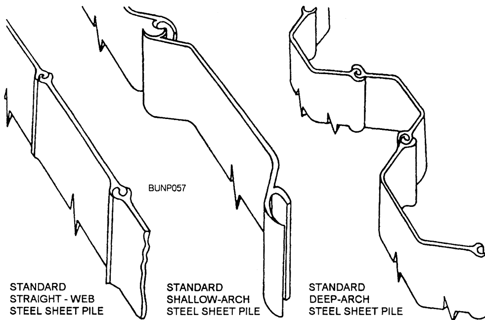
Figure 8-10.—Types of interlocking sheet piles.
