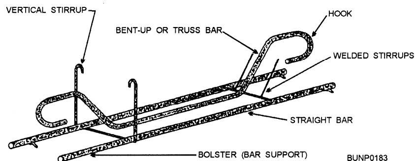
figure 3-11.—Typical shapes of reinforcing steel.
