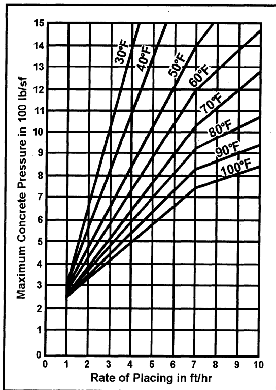
Figure 3-1.—Maximum concrete pressure graph.
