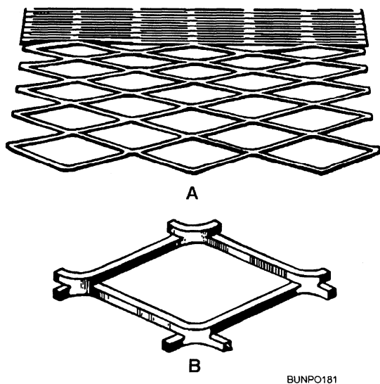
Figure 3-9.—Expanded or diamond mesh steel reinforcement.
