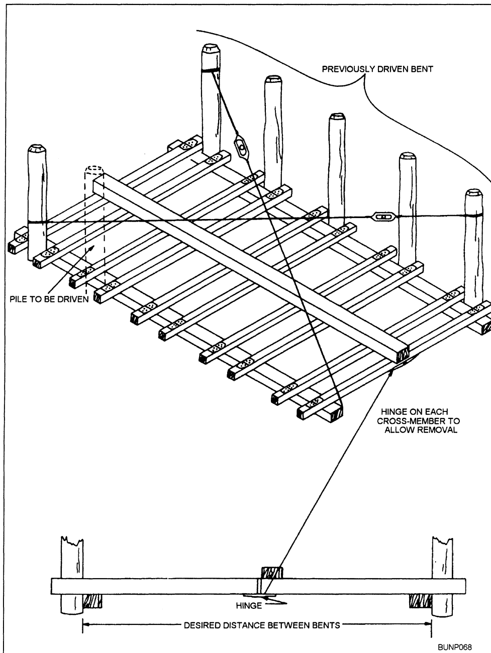
Figure 8-21.—Floating template for positioning piles.
