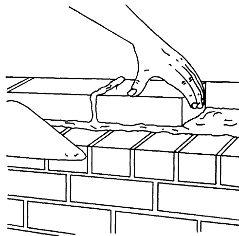
Figure 4-11.—Making a head joint in a stretcher course.
