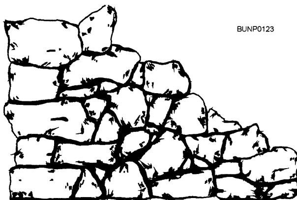
Figure 4-25.—Random rubble stone masonry,
