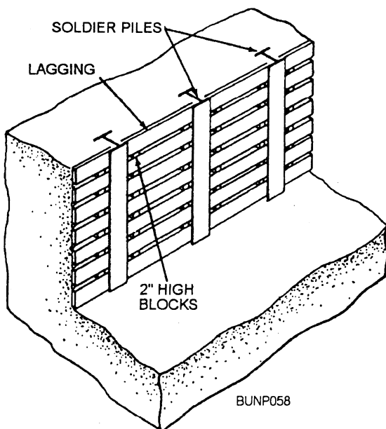
Figure 8-11.—Soldier pile systems.
