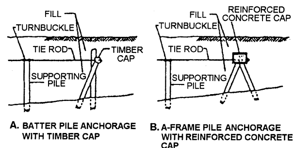
Figure 8-34.—Two types of tie-rod anchorages for bulkheads.
