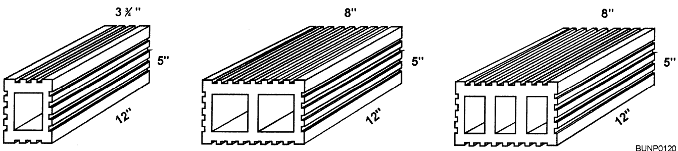
Figure 4-21.—Standard shapes of side-construction building tiles.
