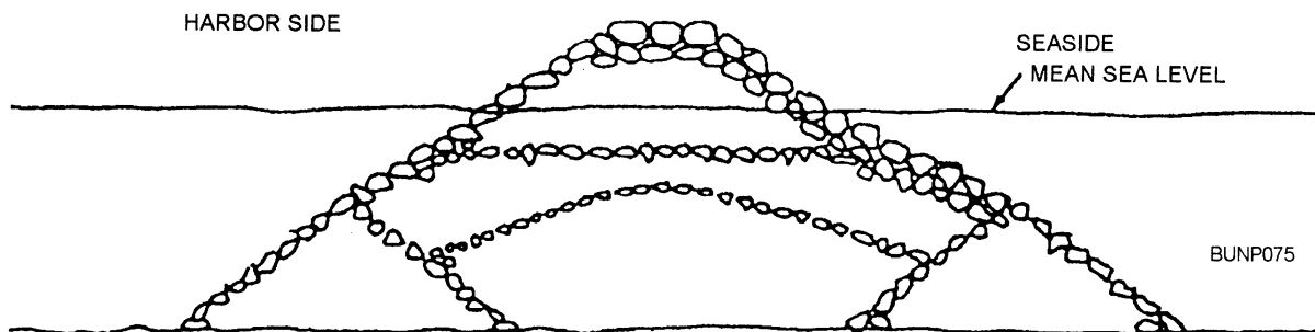
Figure 8-29.—Rubble-mound breakwater or jetty.
