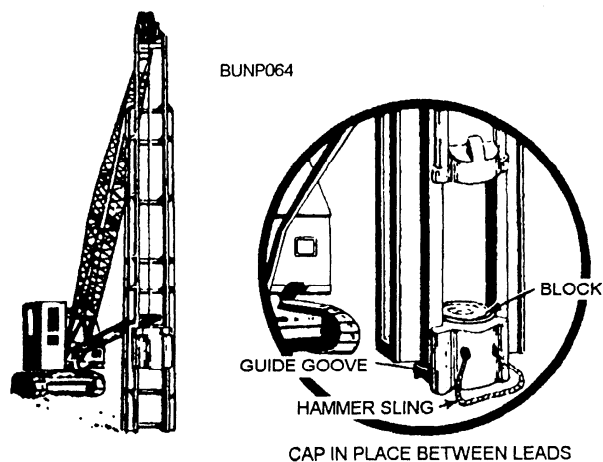
Figure 8-17.—Placing pile cap in leads.
