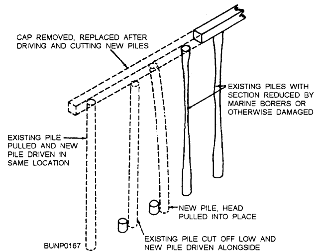
Figure 7-25.—Wood pile replacement.
