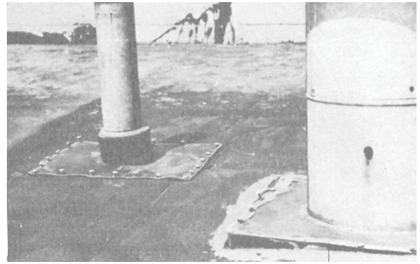
Figure 7-11.—Separation of metal flashing flanged from roof-caused by exposed nails that have worked loose.
