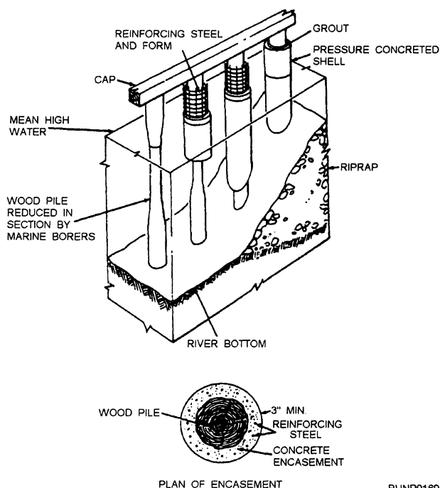
figure 7-27.—Extensive concrete encasement of wood pile.
