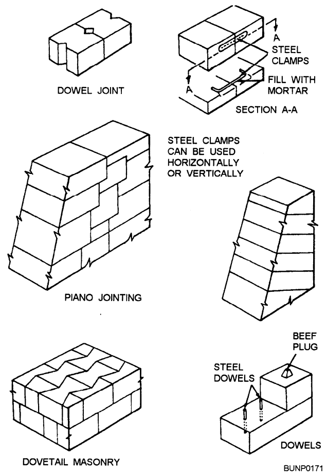
Figure 7-29.—Anchoring masonry blocks.
