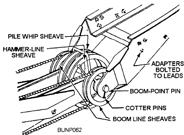
Figure 8-15.—Lead adapters connected to the boom tip.
