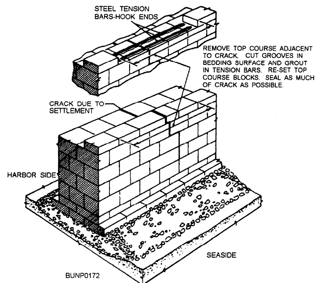
Figure 7-30.—Repair to cracked masonry walls.
