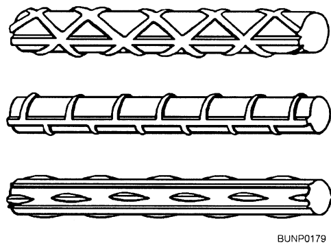
Figure 3-7.—Various types of deformed bar.
