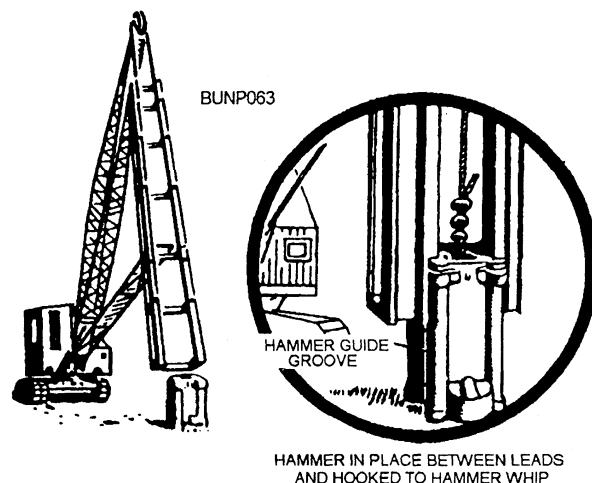
Figure 8-16.—Placing hammer in leads.
