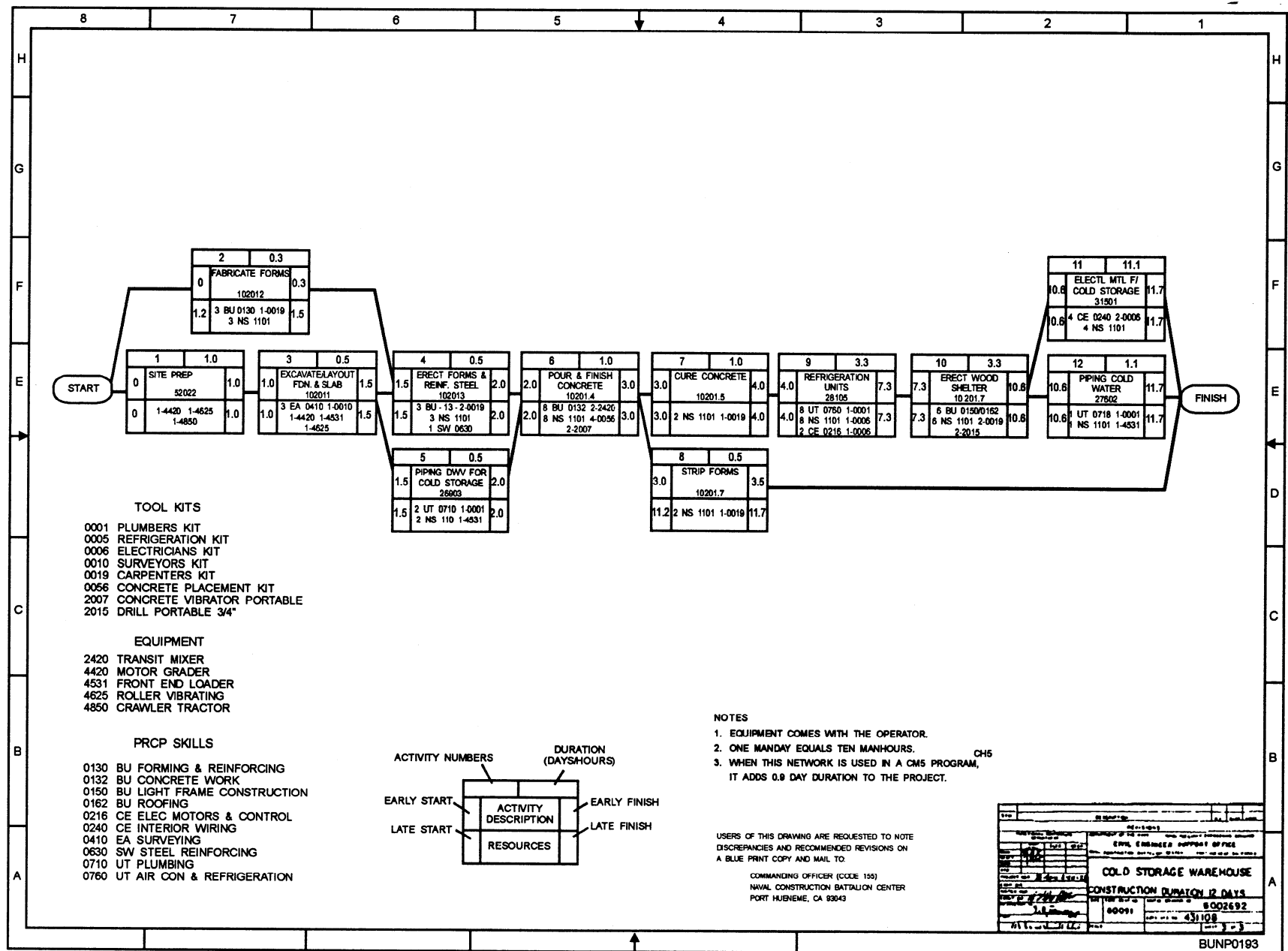
Figure 9-1.—Construction network.
